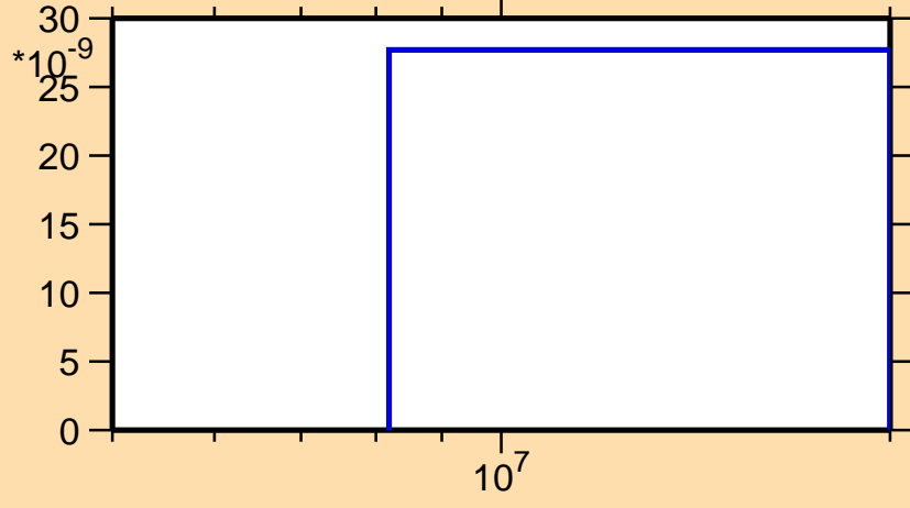
\sigma vs. E for ^{189}\text{Au}(n,nd)
