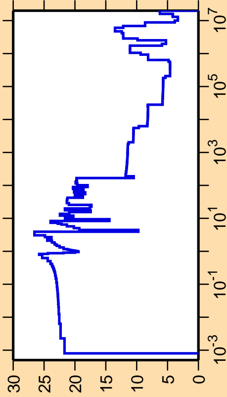
\Delta\sigma/\sigma vs. E for ^{189}\text{Au}(n,\text{el.})
