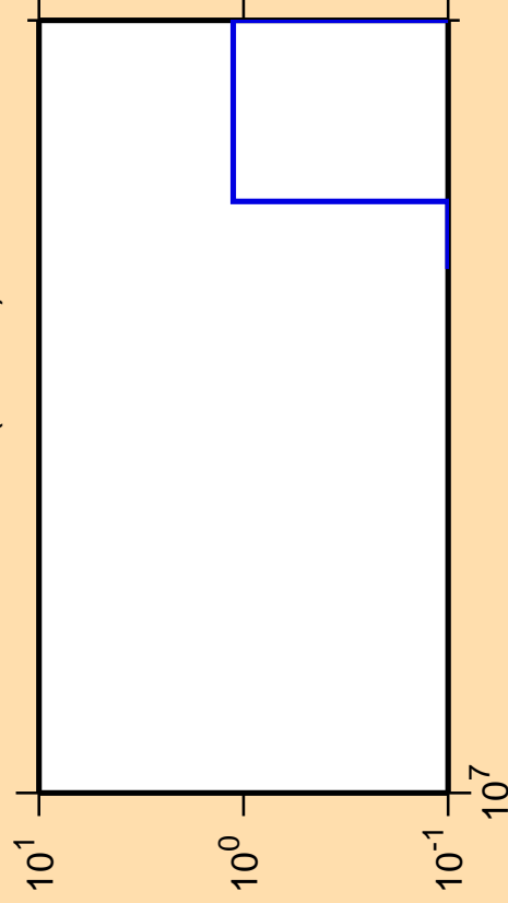
\Delta\sigma/\sigma vs. E for ^{189}\text{Au} (mt 34)
