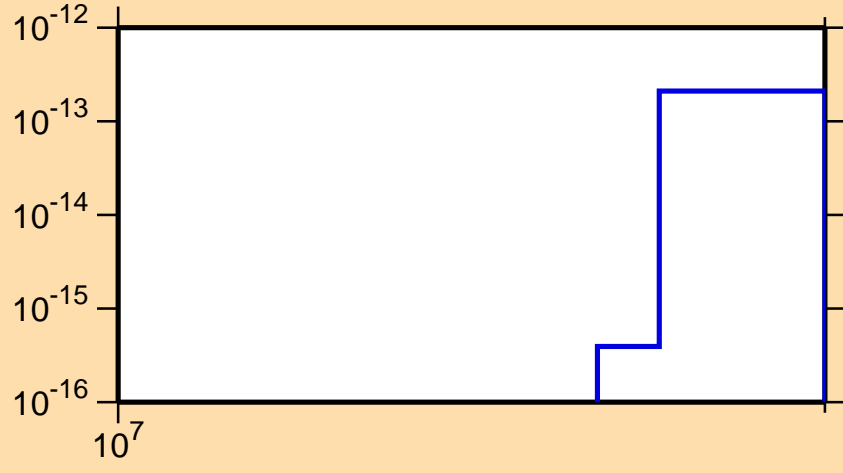
\sigma vs. E for ^{189}\text{Au} (mt 34)
