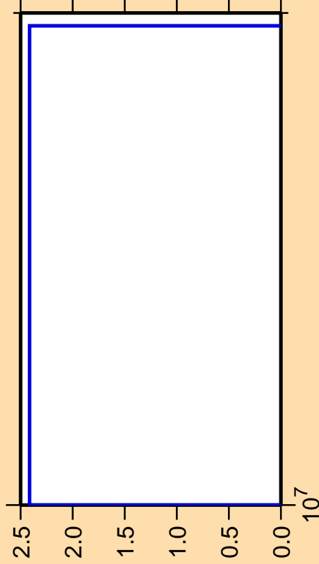
\Delta\sigma/\sigma vs. E for ^{189}\text{Au}(n,3n\alpha)
