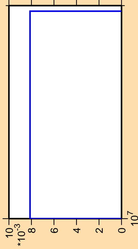
\Delta\sigma/\sigma vs. E for ^{189}\text{Au} (mt 34)
