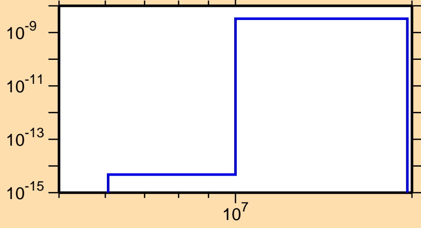
\sigma vs. E for ^{189}\text{Au}(\text{mt } 45)
