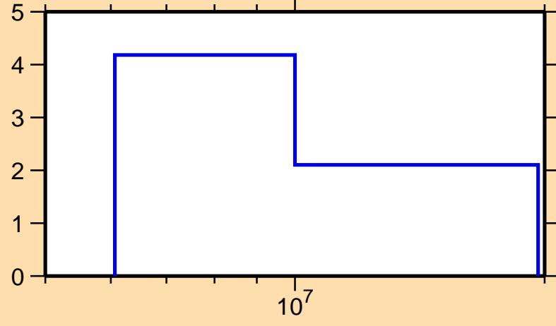
\Delta\sigma/\sigma vs. E for ^{189}\text{Au}(n,\text{tot.})
