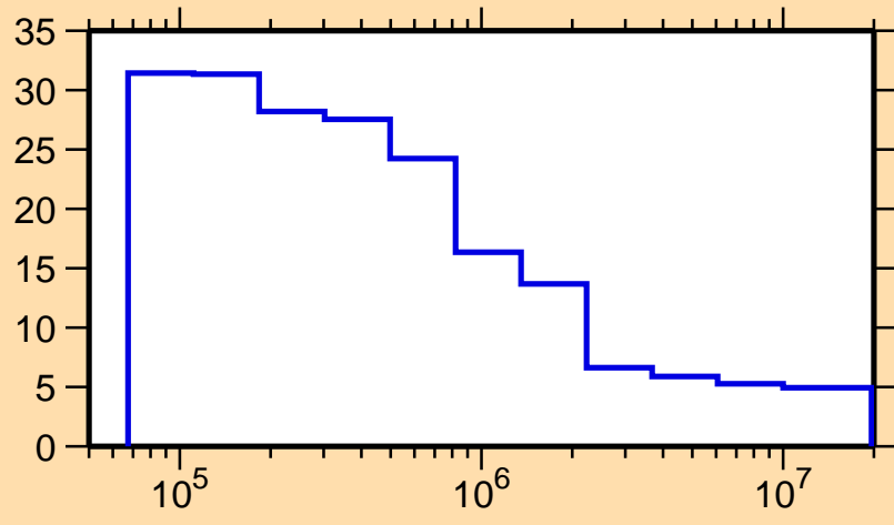
\Delta\sigma/\sigma vs. E for ^{189}\text{Au}(n,\text{nonel.})
