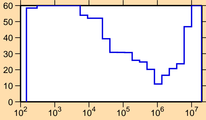
\Delta\sigma/\sigma vs. E for ^{189}\text{Au}(n,\gamma)
