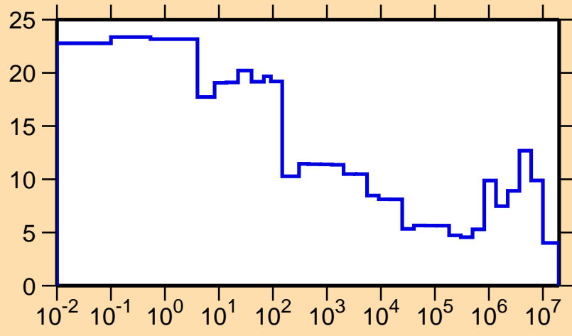
\Delta\sigma/\sigma vs. E for ^{189}\text{Au}(n,\text{el.})
