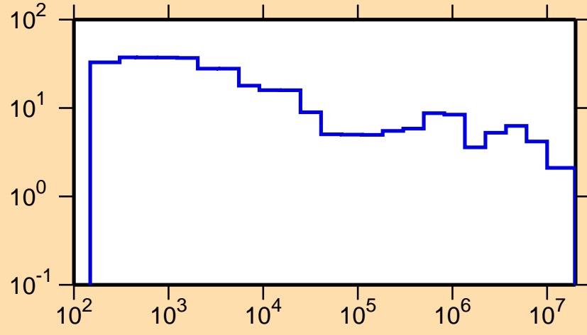
\Delta\sigma/\sigma vs. E for ^{189}\text{Au}(n,\text{tot.})
