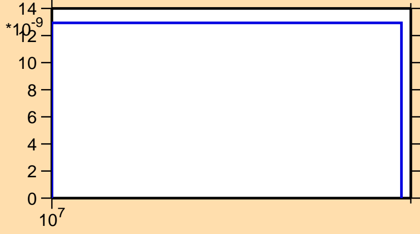
\sigma vs. E for ^{189}\text{Au}(n,\text{nd})
