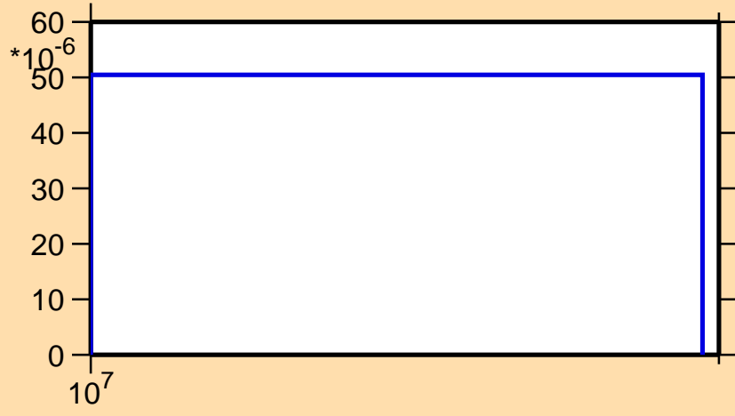
\sigma vs. E for ^{189}\text{Au}(n,3n)
