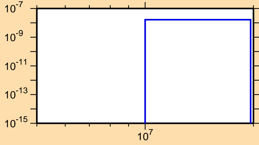
\sigma vs. E for ^{189}\text{Au}(n,\text{He}3)
