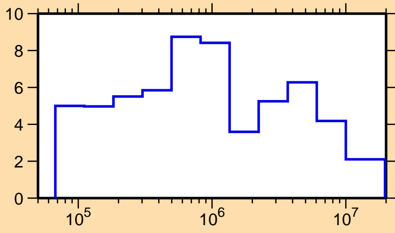
\Delta\sigma/\sigma vs. E for ^{189}\text{Au}(n, \text{tot.})
