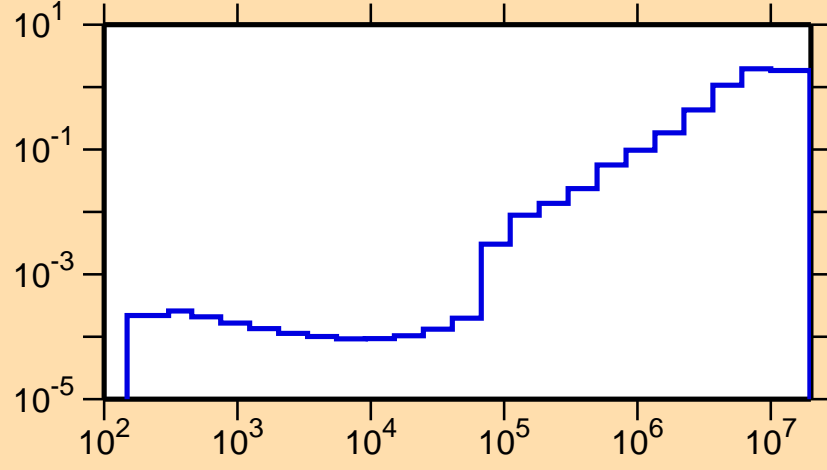
\sigma vs. E for ^{189}\text{Au}(n,\text{inel.})
