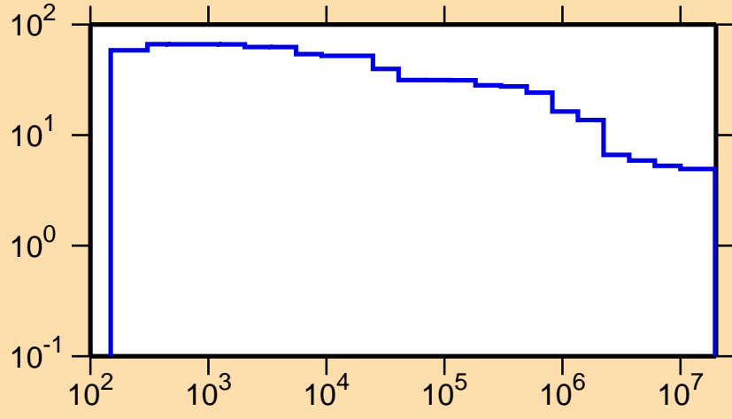
\Delta\sigma/\sigma vs. E for ^{189}\text{Au}(n,\text{nonel.})
