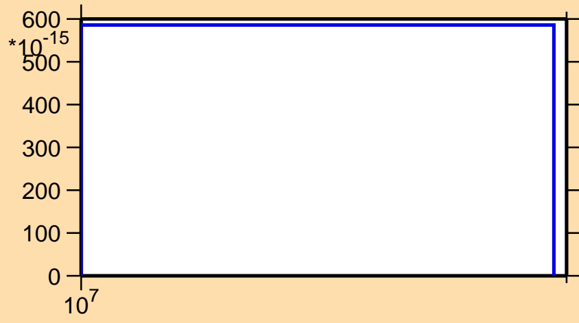
\sigma vs. E for ^{189}\text{Au}(n,3n\alpha)
