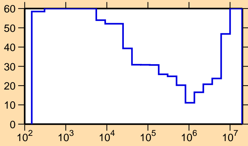
\Delta\sigma/\sigma vs. E for ^{189}\text{Au}(n,\gamma)
