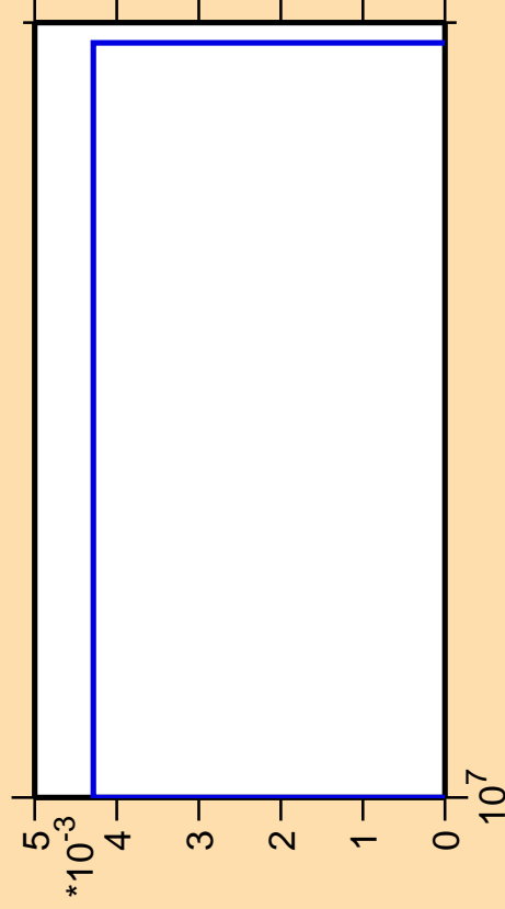
\Delta\sigma/\sigma vs. E for ^{189}\text{Au}(n,\text{pt})
