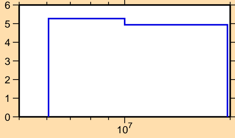
\Delta\sigma/\sigma vs. E for ^{189}\text{Au}(n,\text{nonel.})
