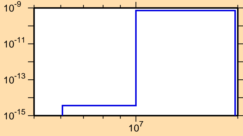
\sigma vs. E for ^{189}\text{Au}(\text{mt117})
