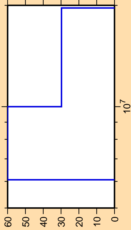
\Delta\sigma/\sigma vs. E for ^{189}\text{Au}(n,2n)
