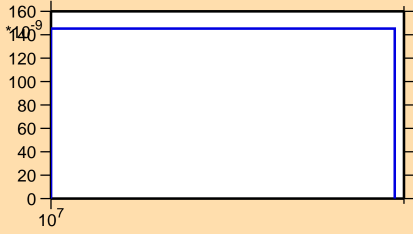
\sigma vs. E for ^{189}\text{Au}(n,2np)
