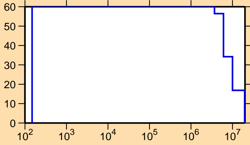
\Delta\sigma/\sigma vs. E for ^{189}\text{Au}(n,p)
