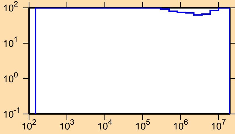
\Delta\sigma/\sigma vs. E for ^{189}\text{Au}(n,n_1)
