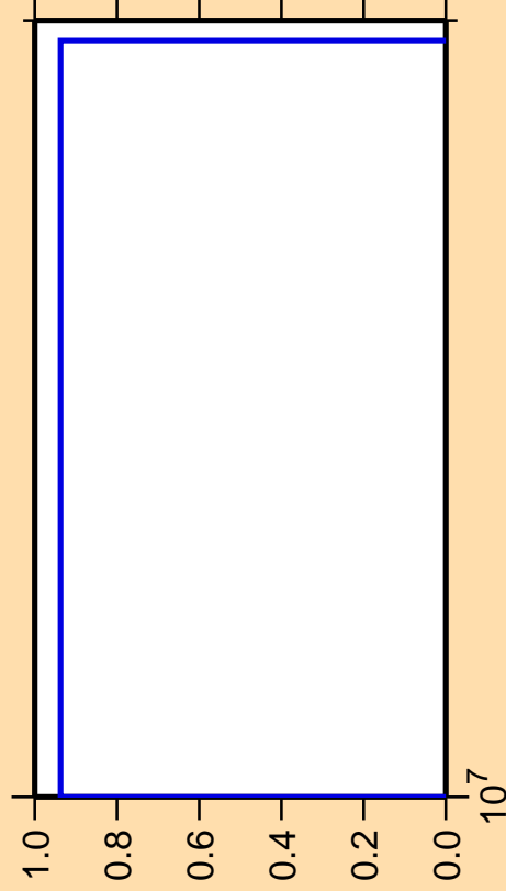
\Delta\sigma/\sigma vs. E for ^{189}\text{Au}(n,\text{pd})
