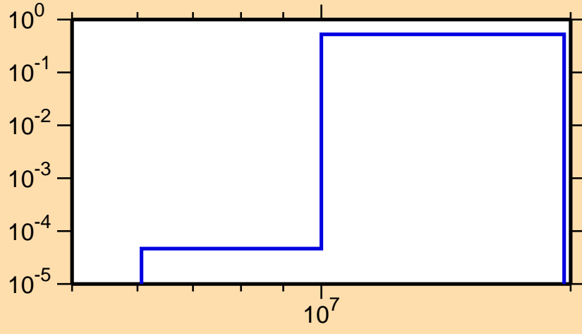
\sigma vs. E for ^{189}\text{Au}(n,2n)
