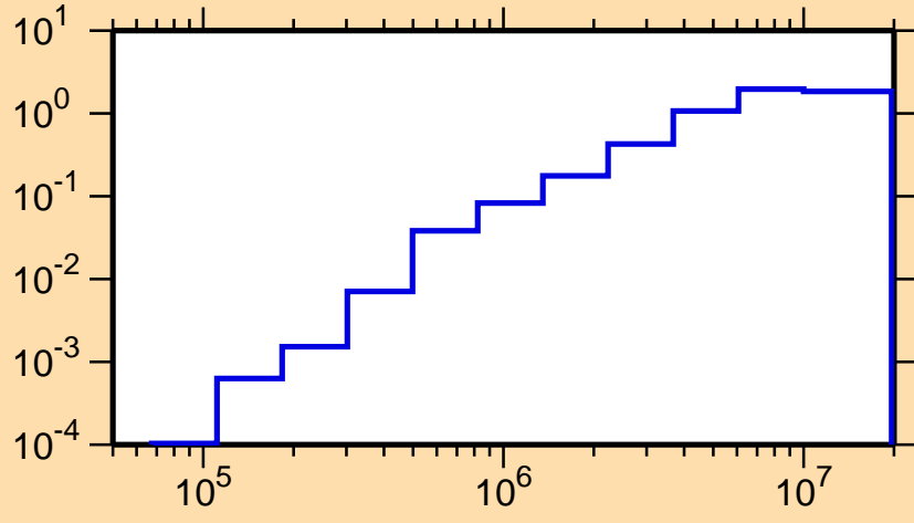
\sigma vs. E for ^{189}\text{Au}(n,n\text{cont.})
