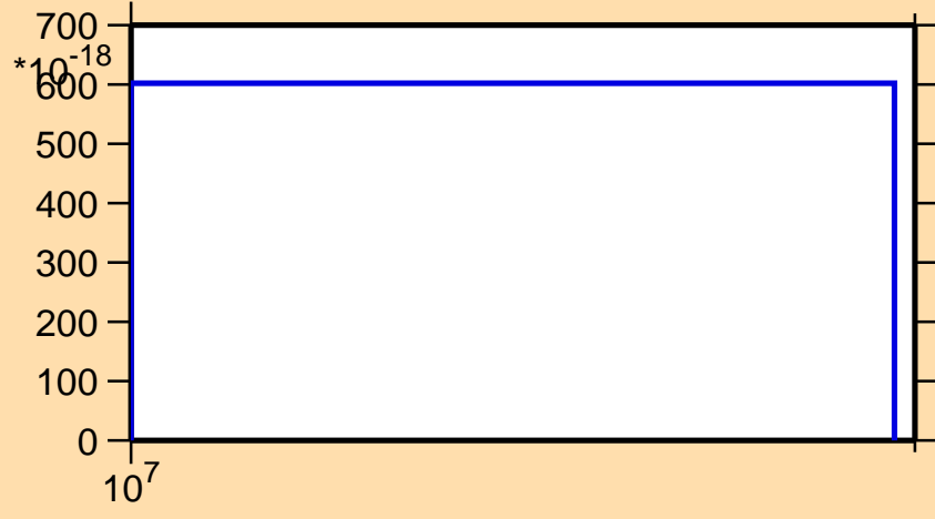
\sigma vs. E for ^{189}\text{Au}(n,\text{pt})
