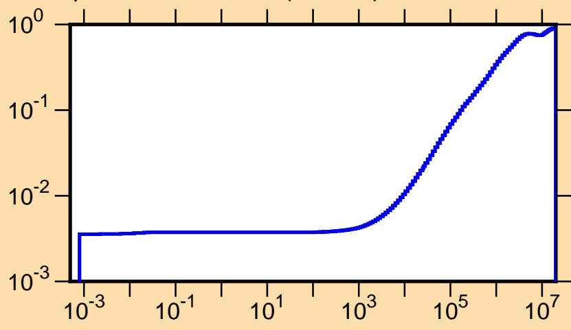
\mu vs. E for ^{190}\text{Au}(\text{mt251})
