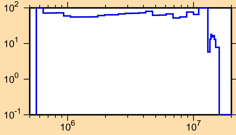
\Delta\sigma/\sigma vs. E for ^{190}\text{Au}(n,n_1)
