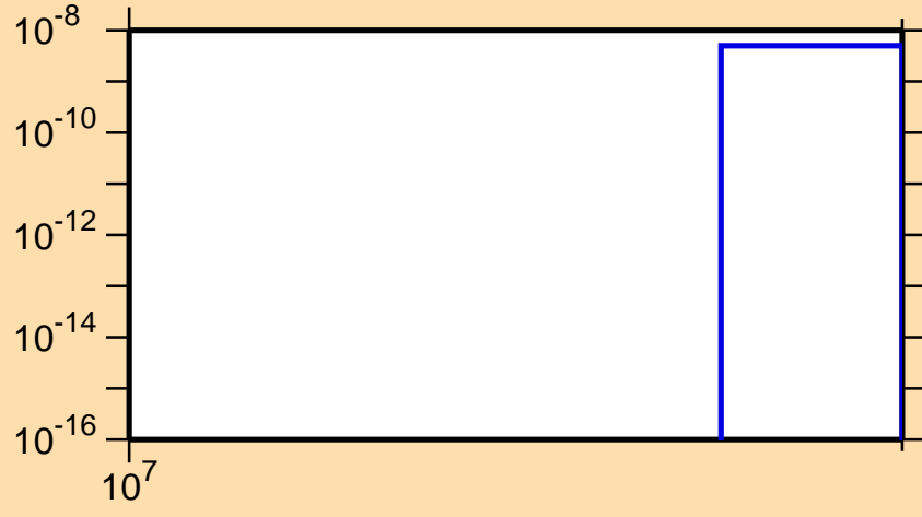
\sigma vs. E for ^{190}\text{Au}(n,3n\alpha)
