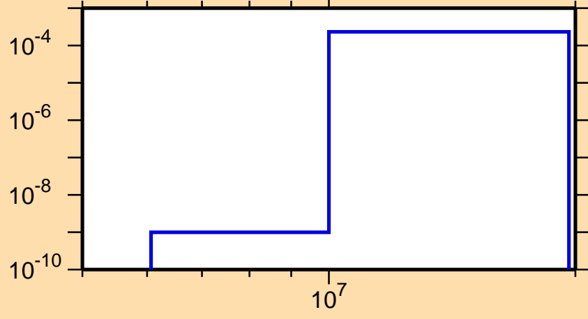
\sigma vs. E for ^{190}\text{Au}(n,t)
