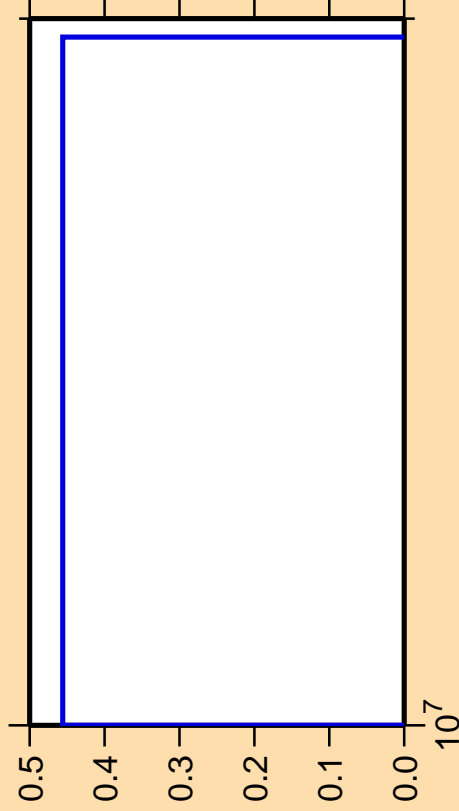
\Delta\sigma/\sigma vs. E for ^{190}\text{Au} (mt 34)
