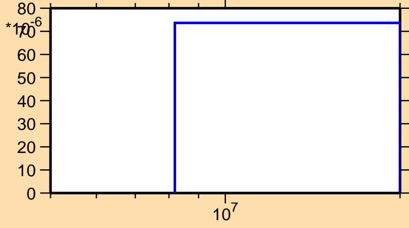
\sigma vs. E for ^{190}\text{Au}(n,3n)
