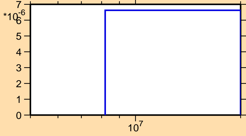
\sigma vs. E for ^{190}\text{Au}(n,2np)
