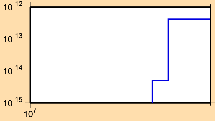
\sigma vs. E for ^{191}\text{Au}(n,\text{pd})
