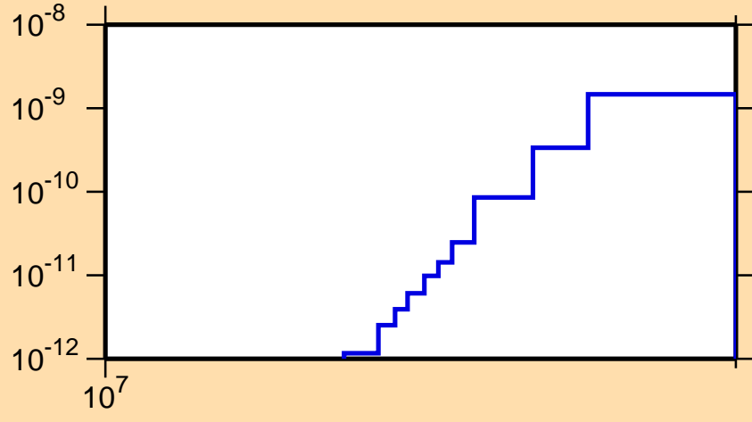
\sigma vs. E for ^{191}\text{Au}(\text{mt117})
