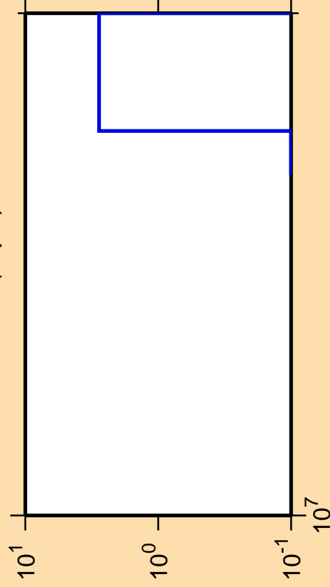
\Delta\sigma/\sigma vs. E for ^{191}\text{Au}(n,\text{pd})
