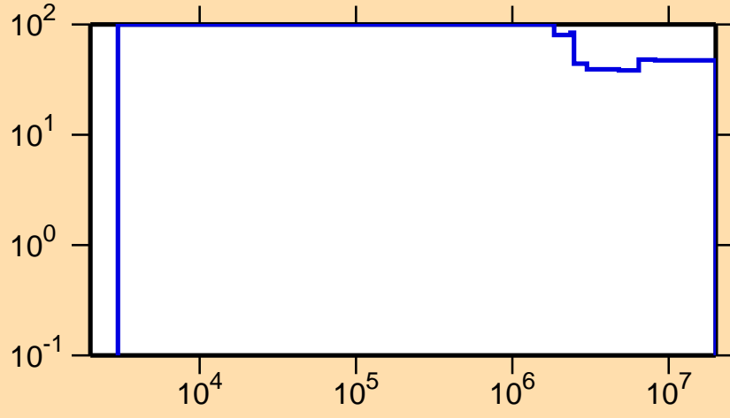
\Delta\sigma/\sigma vs. E for ^{191}\text{Au}(n,n_1)
