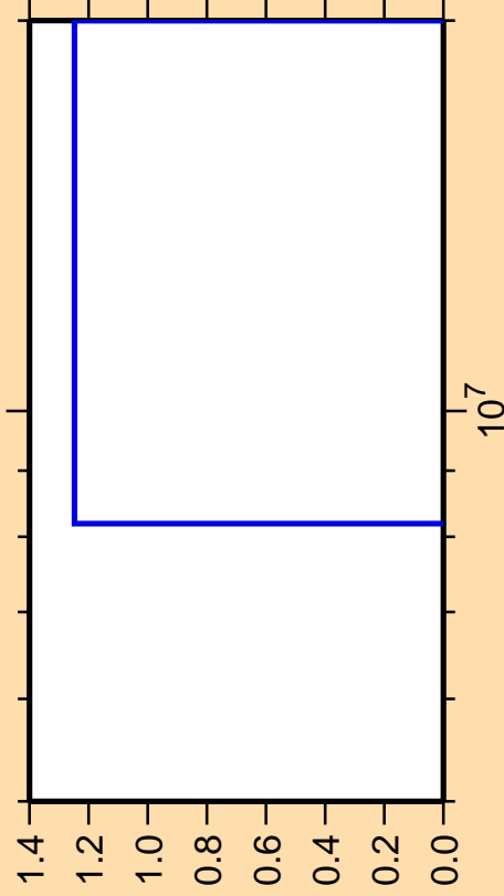
\Delta\sigma/\sigma vs. E for ^{191}\text{Au}(n,3n\alpha)
