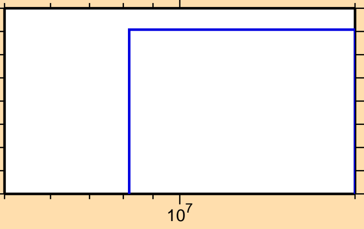
\sigma vs. E for ^{191}\text{Au}(n,t)
