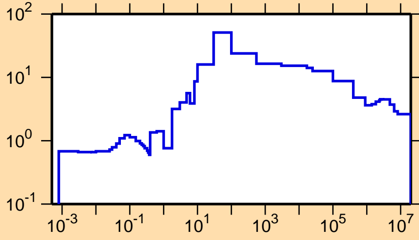
\sigma vs. E for ^{191}\text{Au}(n,\text{el.})
