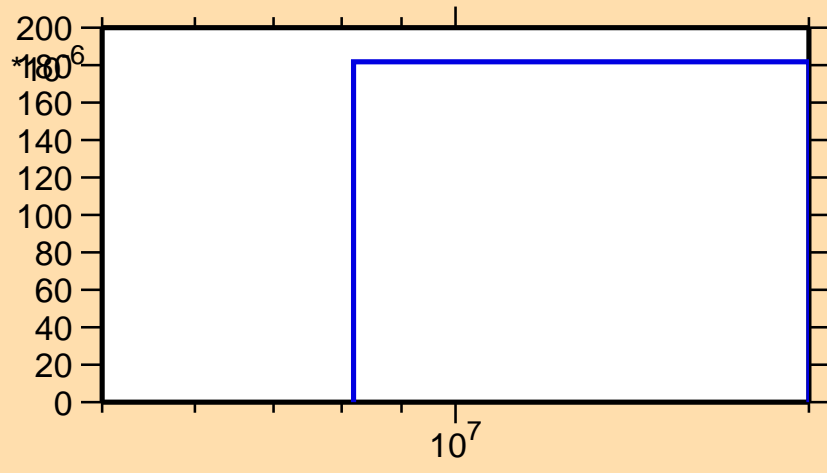
\sigma vs. E for ^{191}\text{Au}(n,3n)
