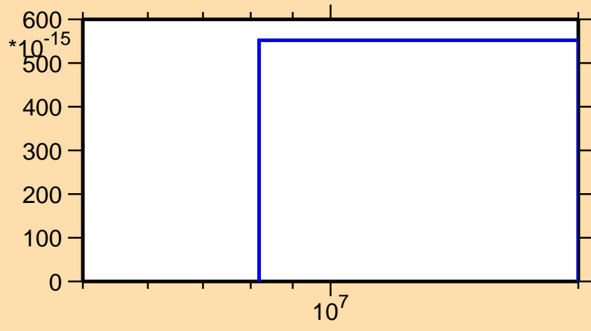
\sigma vs. E for ^{191}\text{Au}(n,3n\alpha)
