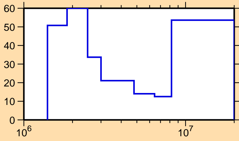
\Delta\sigma/\sigma vs. E for ^{191}\text{Au}(n,n\text{cont.})
