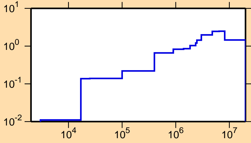
\sigma vs. E for ^{191}\text{Au}(n,\text{inel.})
