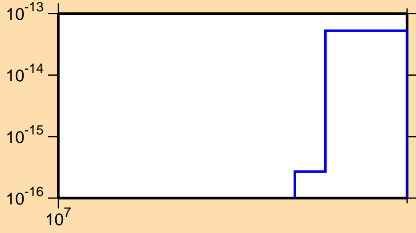
\sigma vs. E for ^{192}\text{Au}(n,\text{pd})
