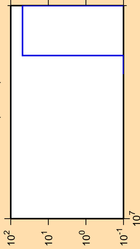
\Delta\sigma/\sigma vs. E for ^{192}\text{Au}(n,3n\alpha)
