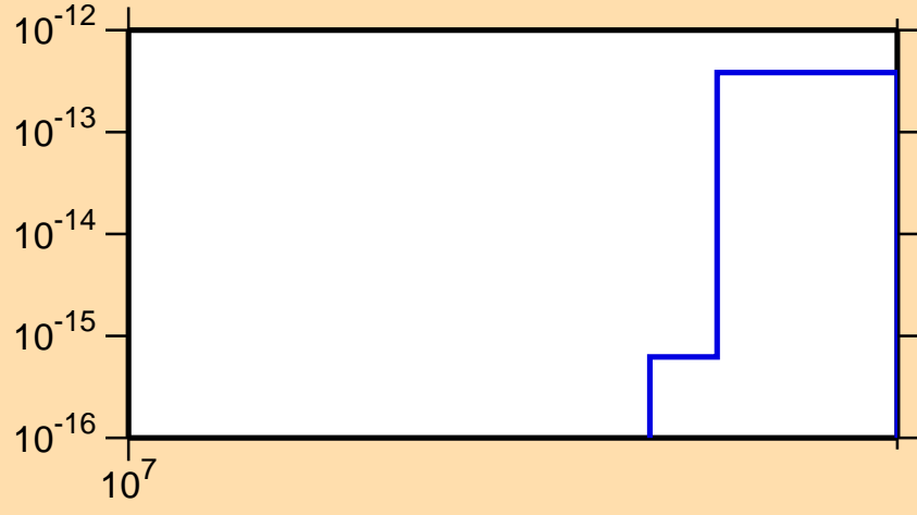
\sigma vs. E for ^{192}\text{Au} (mt 34)
