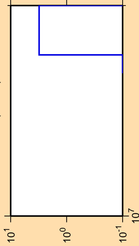
\Delta\sigma/\sigma vs. E for ^{192}\text{Au} (mt 34)
