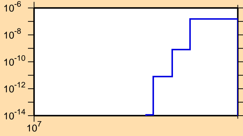
\sigma vs. E for ^{192}\text{Au}(n,nt)
