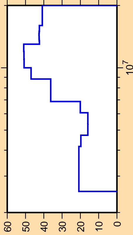
\Delta\sigma/\sigma vs. E for ^{192}\text{Au}(n,n\text{cont.})
