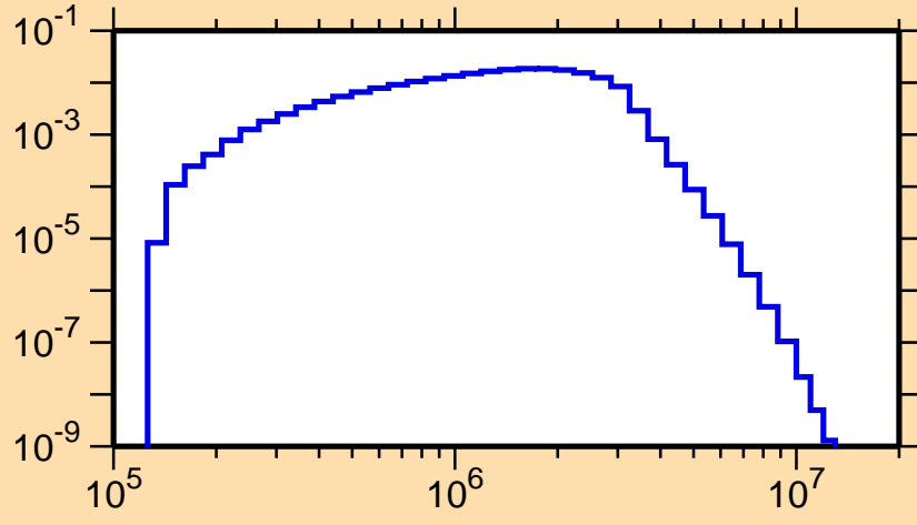
\sigma vs. E for ^{192}\text{Au}(n,n_4)
