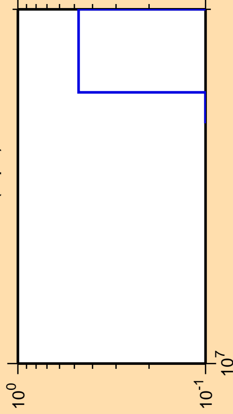
\Delta\sigma/\sigma vs. E for ^{192}\text{Au}(n,\text{pd})
