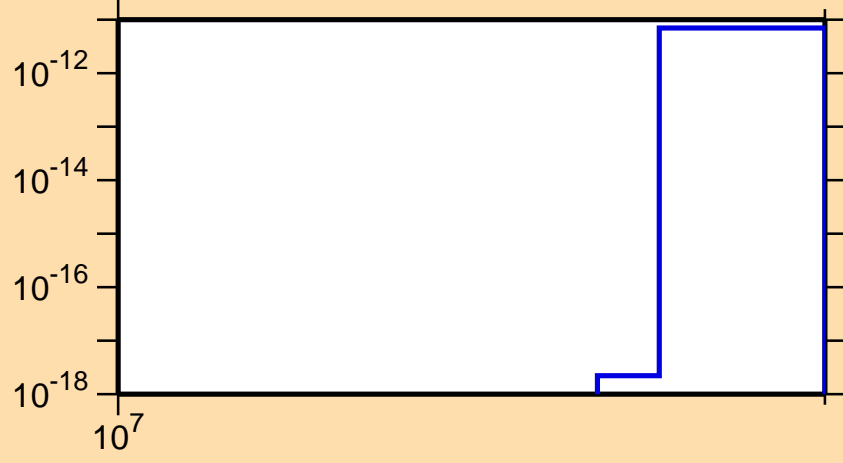
\sigma vs. E for ^{192}\text{Au}(n,3n\alpha)
