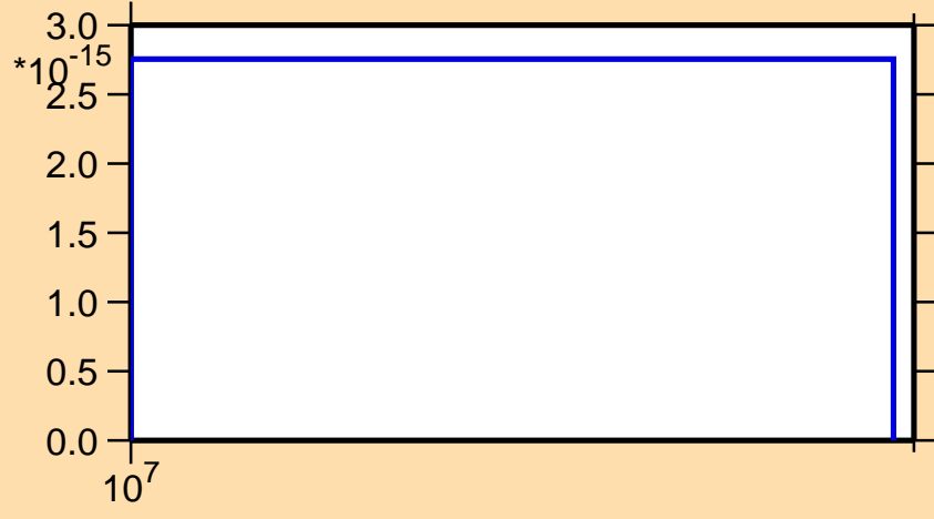
\sigma vs. E for ^{192}\text{Au} (mt 34)
