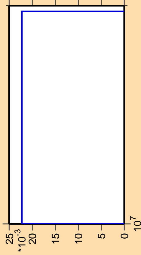
\Delta\sigma/\sigma vs. E for ^{192}\text{Au} (mt 34)
