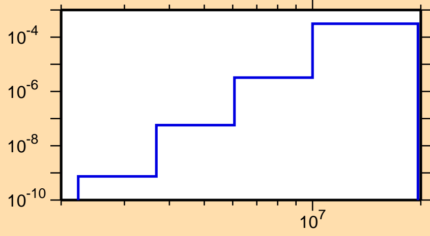
\sigma vs. E for ^{192}\text{Au}(n,n\alpha)
