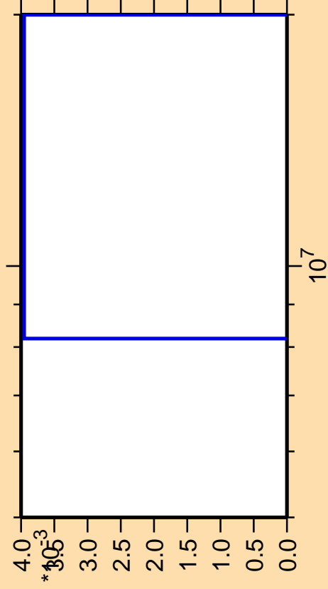
\Delta\sigma/\sigma vs. E for ^{192}\text{Au}(n,pd)
