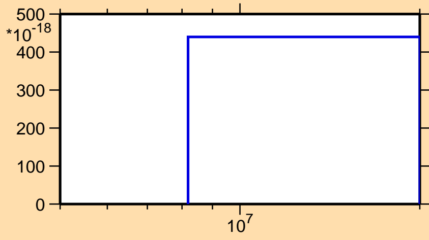
\sigma vs. E for ^{192}\text{Au}(n,pd)
