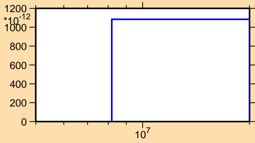
\sigma vs. E for ^{192}\text{Au}(n,\text{He3})
