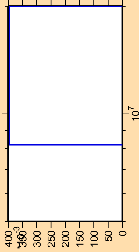
\Delta\sigma/\sigma vs. E for ^{192}\text{Au}(n,3n\alpha)
