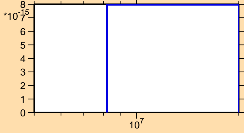
\sigma vs. E for ^{193}\text{Au}(n,3n\alpha)
