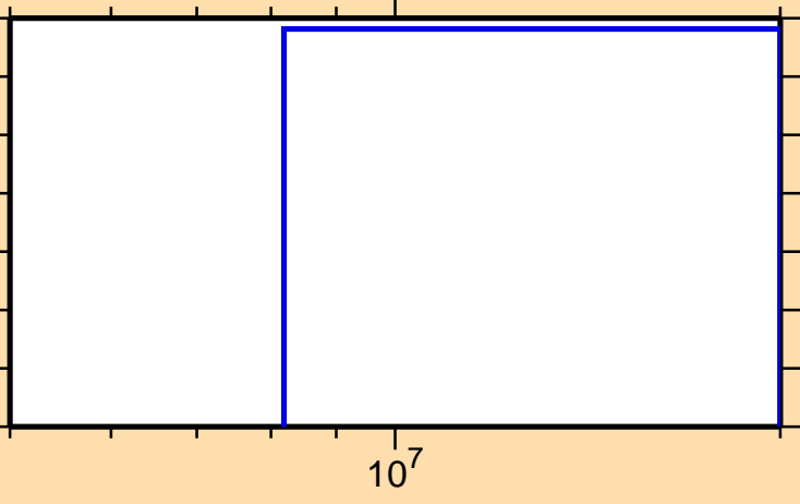
\sigma vs. E for ^{193}\text{Au}(n,\text{nd})
