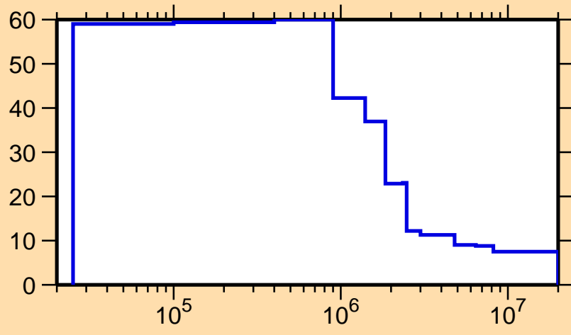
\Delta\sigma/\sigma vs. E for ^{193}\text{Au}(n,\text{nonel.})
