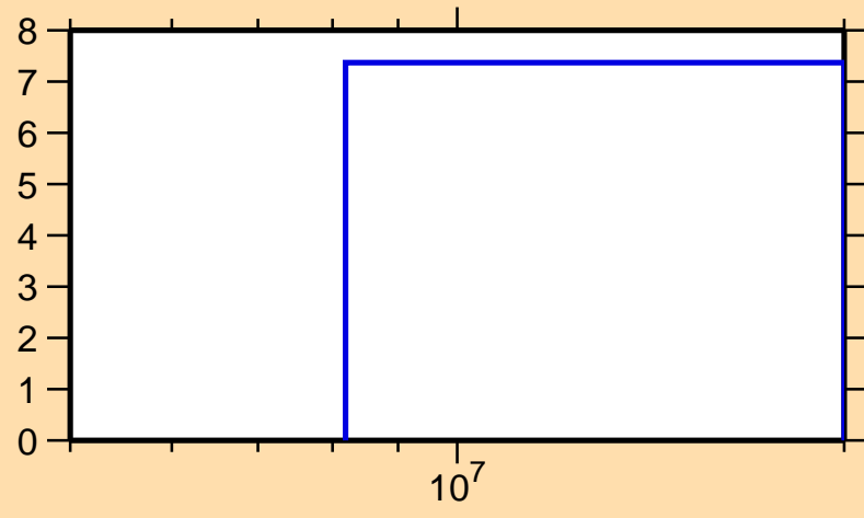
\Delta\sigma/\sigma vs. E for ^{193}\text{Au}(n,\text{el.})
