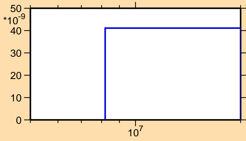
\sigma vs. E for ^{193}\text{Au}(n,2n\alpha)
