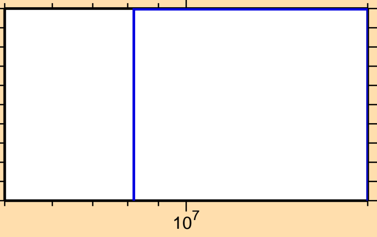
\sigma vs. E for ^{193}\text{Au}(n,t)
