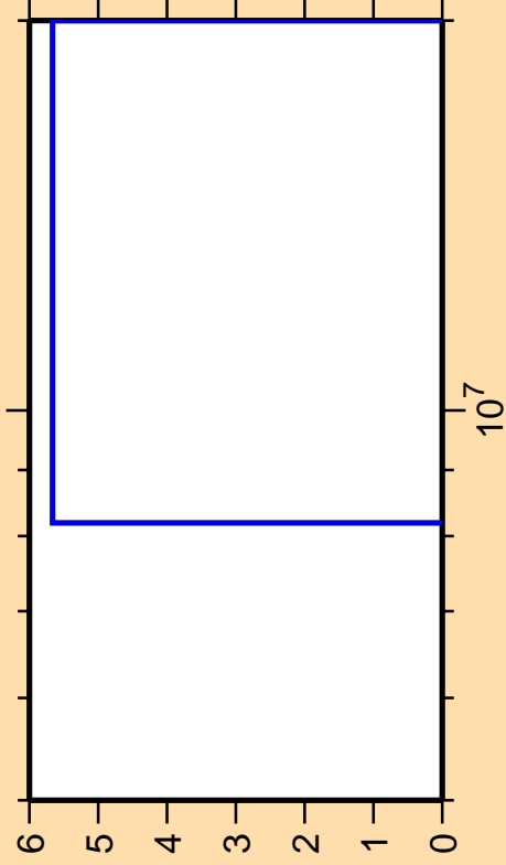
\Delta\sigma/\sigma vs. E for ^{193}\text{Au}(\text{mt } 45)
