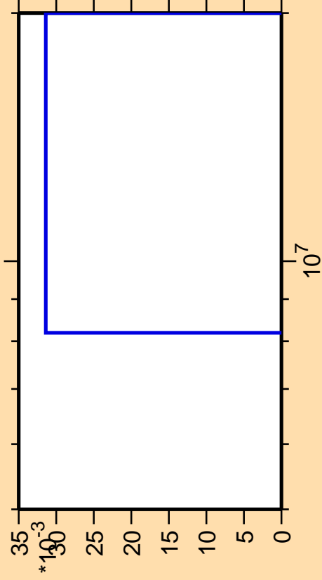
\Delta\sigma/\sigma vs. E for ^{193}\text{Au}(n,3n\alpha)
