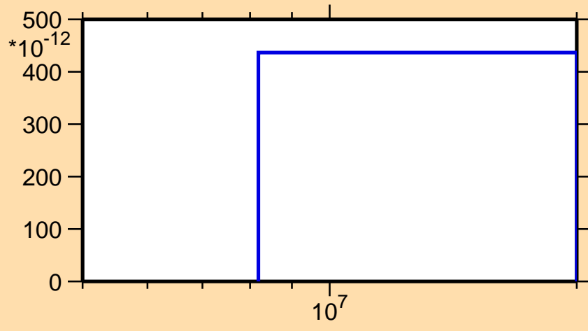
\sigma vs. E for ^{193}\text{Au}(n,p\alpha)
