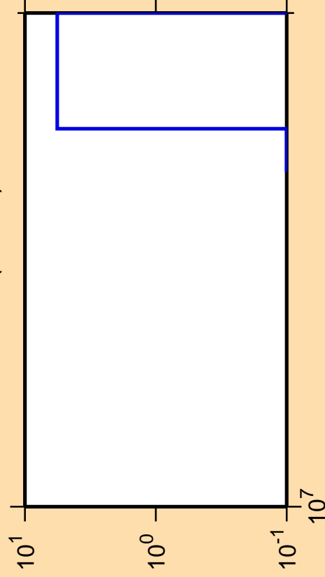
\Delta\sigma/\sigma vs. E for ^{193}\text{Au}(n,3n\alpha)
