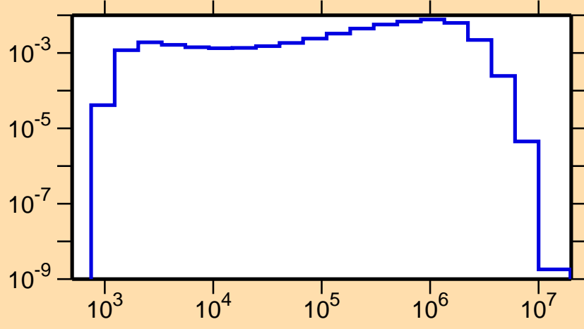
\sigma vs. E for ^{193}\text{Au}(n,n_1)
