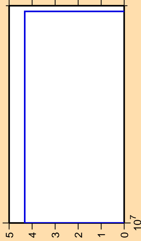
\Delta\sigma/\sigma vs. E for ^{193}\text{Au} (mt 45)
