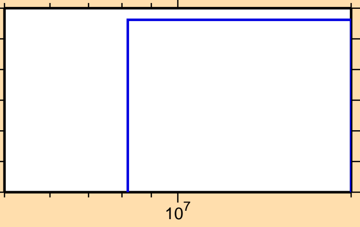
\sigma vs. E for ^{193}\text{Au}(n,2n\alpha)
