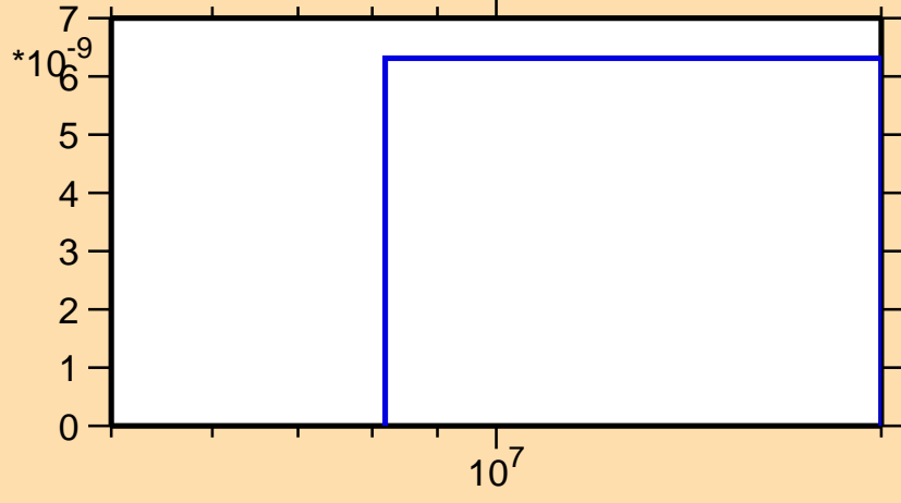
\sigma vs. E for ^{193}\text{Au}(n,nd)
