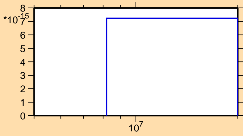
\sigma vs. E for ^{193}\text{Au}(n,3n\alpha)
