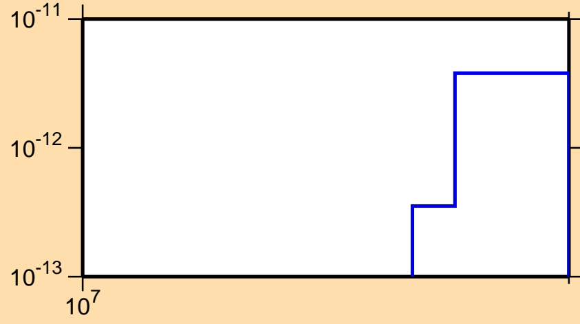
\sigma vs. E for ^{194}\text{Au}(\text{mt } 45)
