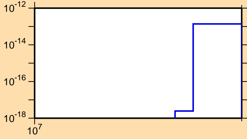
\sigma vs. E for ^{194}\text{Au}(n,3n\alpha)
