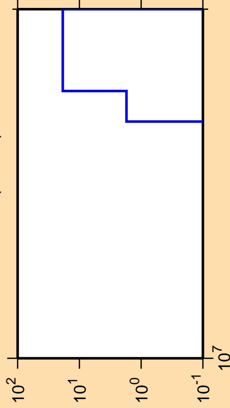
\Delta\sigma/\sigma vs. E for ^{194}\text{Au}(\text{mt } 45)
