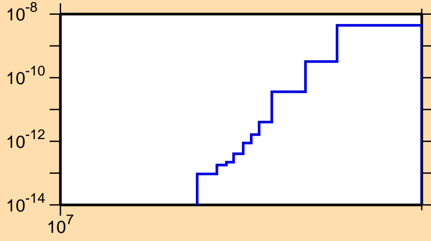
\sigma vs. E for ^{194}\text{Au}(n,\text{He3})
