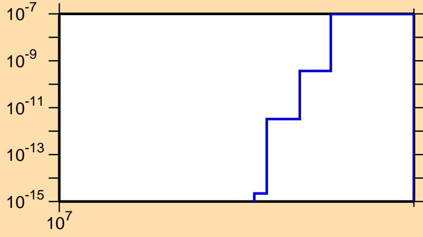
\sigma vs. E for ^{194}\text{Au}(n,nt)
