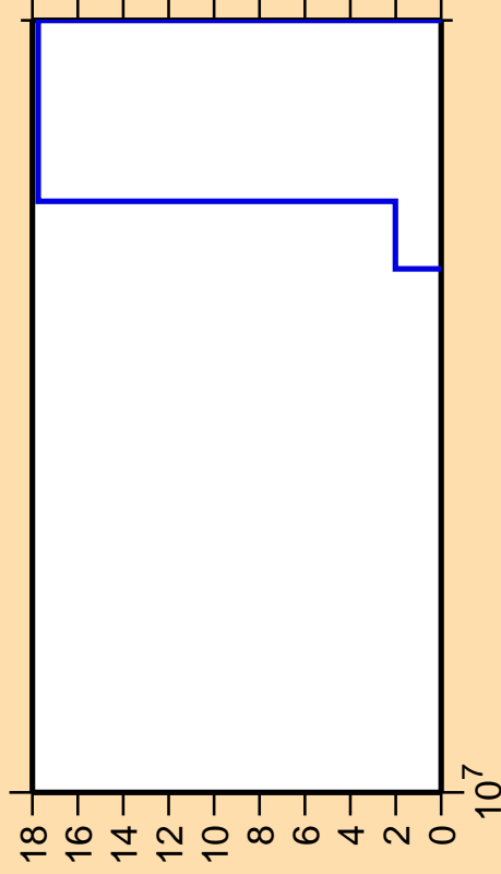
\Delta\sigma/\sigma vs. E for ^{194}\text{Au}(\text{mt117})
