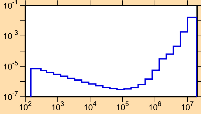
\sigma vs. E for ^{194}\text{Au}(n,p)
