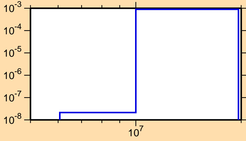
\sigma vs. E for ^{194}\text{Au}(n,d)
