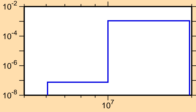
\sigma vs. E for ^{194}\text{Au}(n,np)
