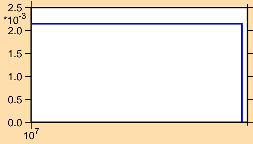
\sigma vs. E for ^{194}\text{Au}(n,3n)
