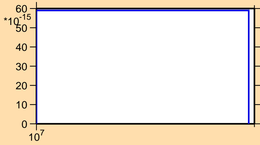
\sigma vs. E for ^{194}\text{Au}(\text{mt117})
