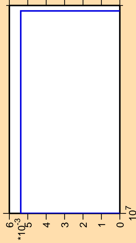
\Delta\sigma/\sigma vs. E for ^{194}\text{Au}(n,3n\alpha)
