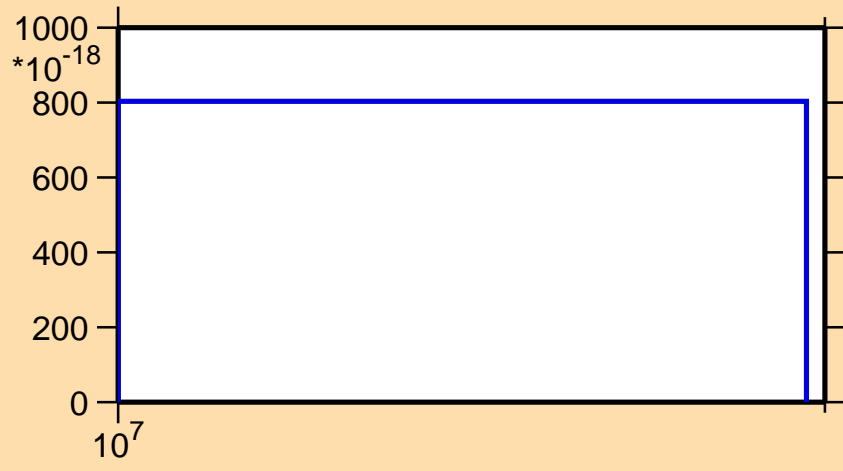
\sigma vs. E for ^{194}\text{Au}(n,3n\alpha)
