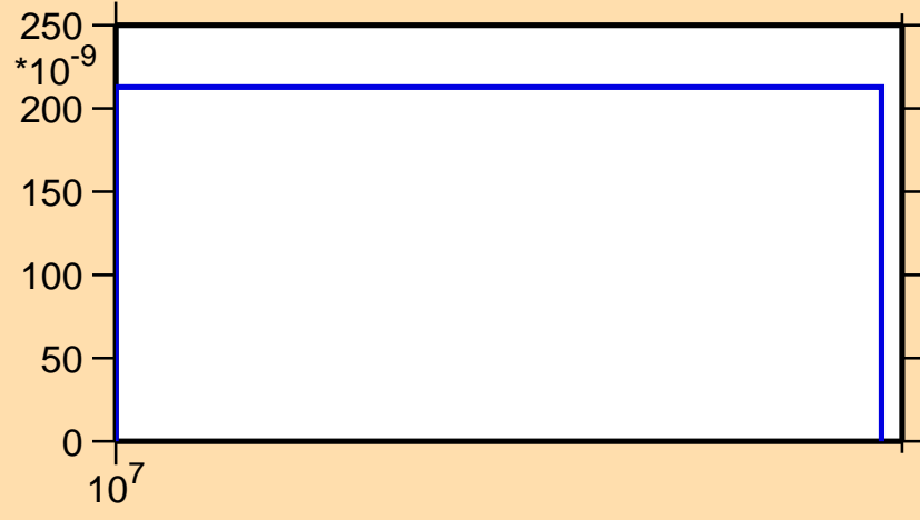
\sigma vs. E for ^{194}\text{Au}(n,2np)
