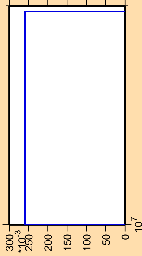
\Delta\sigma/\sigma vs. E for ^{194}\text{Au}(\text{mt } 45)
