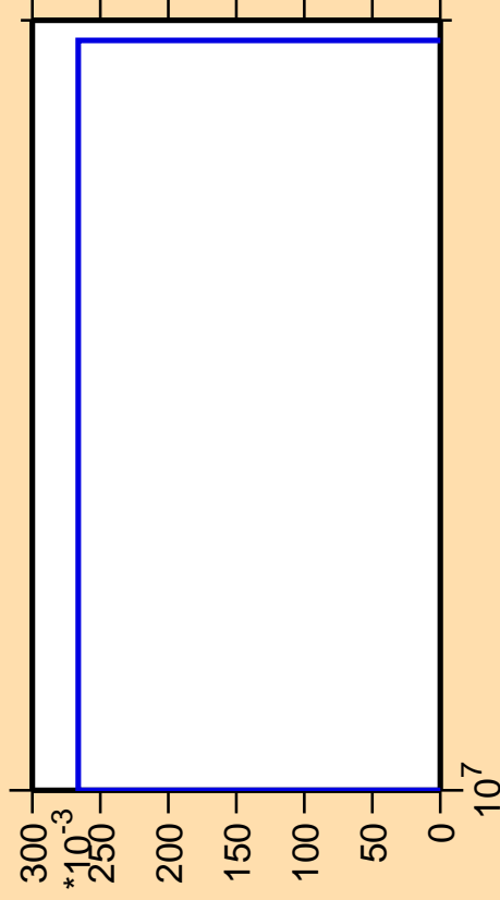
\Delta\sigma/\sigma vs. E for ^{194}\text{Au}(\text{mt117})
