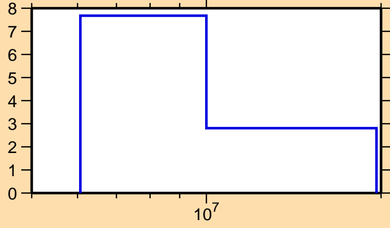
\Delta\sigma/\sigma vs. E for ^{194}\text{Au}(n,\text{tot.})
