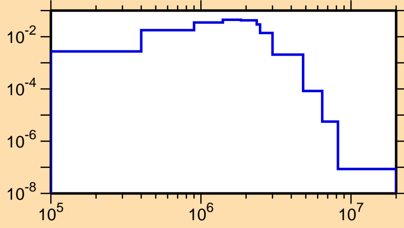
\sigma vs. E for ^{194}\text{Au}(n,n_3)
