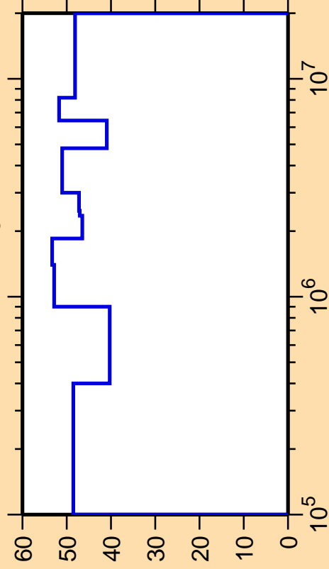
\Delta\sigma/\sigma vs. E for ^{194}\text{Au}(n,n_3)
