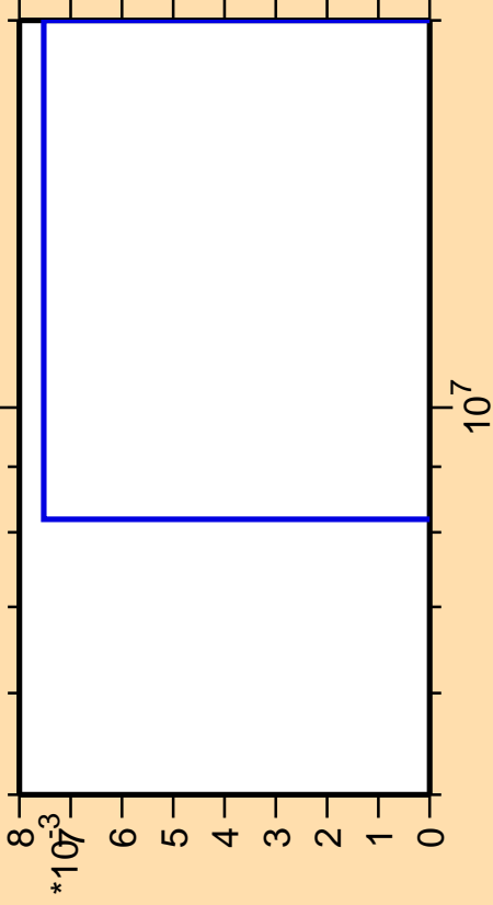
\Delta\sigma/\sigma vs. E for ^{194}\text{Au}(n,3n\alpha)
