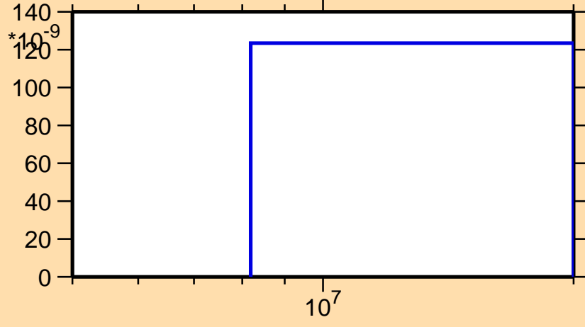
\sigma vs. E for ^{194}\text{Au}(n,nd)
