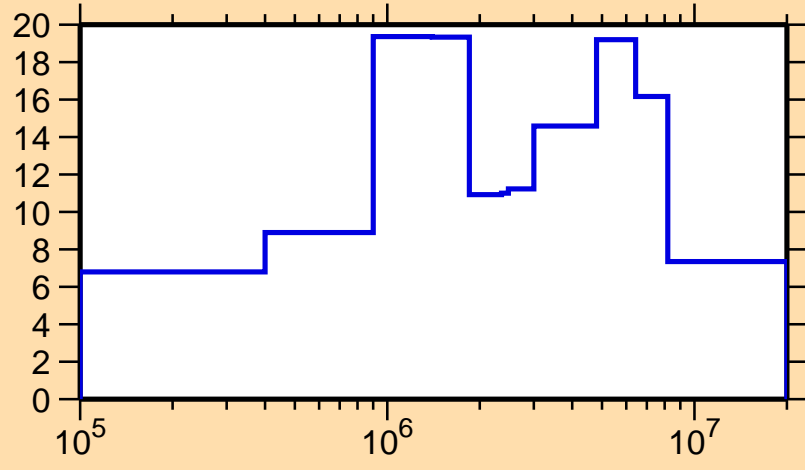
\Delta\sigma/\sigma vs. E for ^{194}\text{Au}(n, el.)
