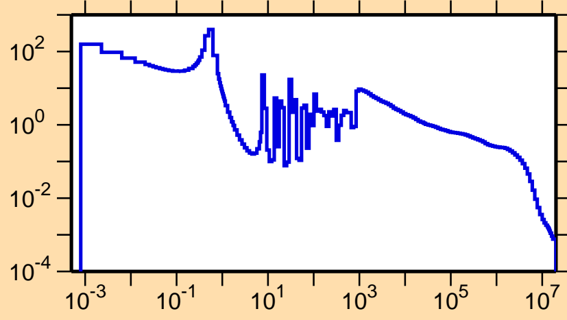
\sigma vs. E for ^{195}\text{Au}(n,\gamma)
