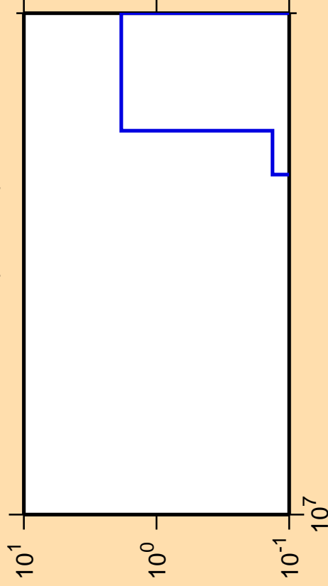
\Delta\sigma/\sigma vs. E for ^{195}\text{Au}(\text{mt117})
