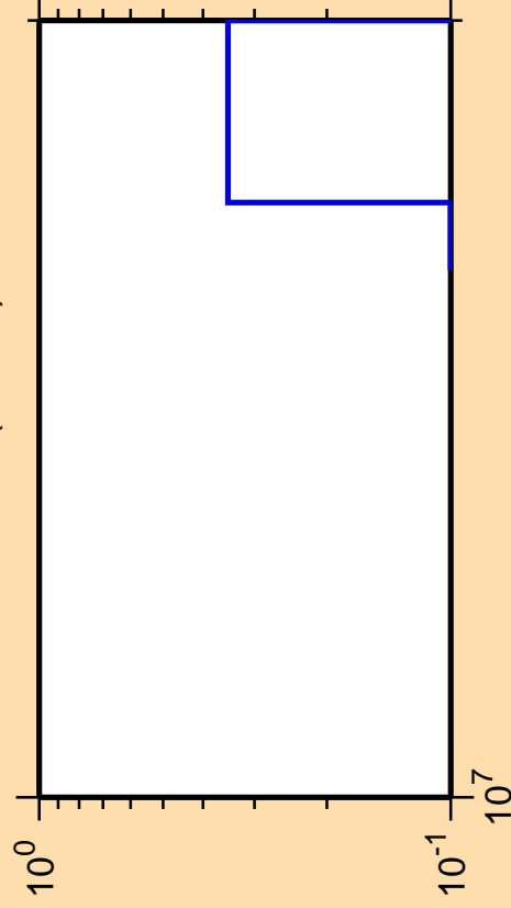
\Delta\sigma/\sigma vs. E for ^{195}\text{Au}(\text{mt } 45)
