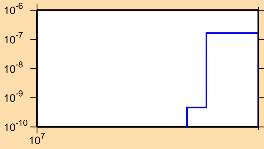
\sigma vs. E for ^{195}\text{Au}(n,2np)
