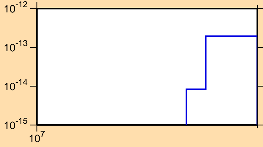
\sigma vs. E for ^{195}\text{Au}(\text{mt } 45)
