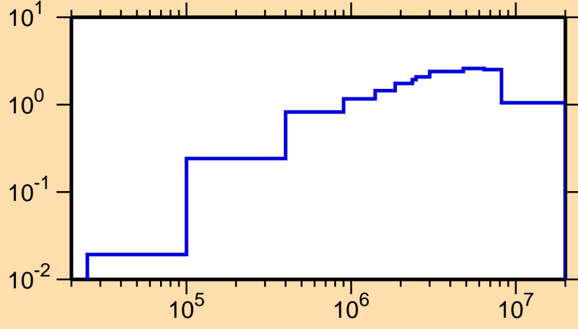
\sigma vs. E for ^{195}\text{Au}(n,\text{inel.})
