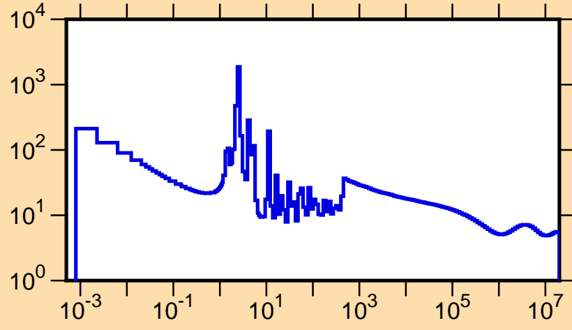
\sigma vs. E for ^{196}\text{Au}(n,\text{tot.})
