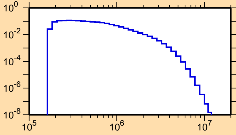
\sigma vs. E for ^{196}\text{Au}(n,n_4)
