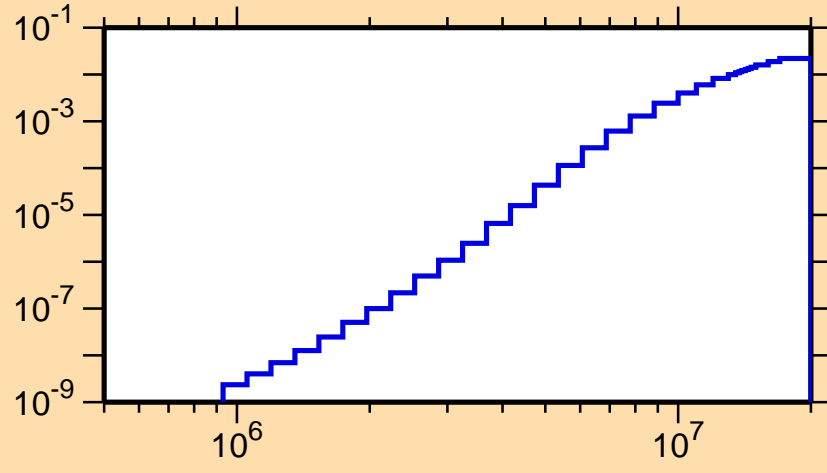
\sigma vs. E for ^{196}\text{Au}(n,p)
