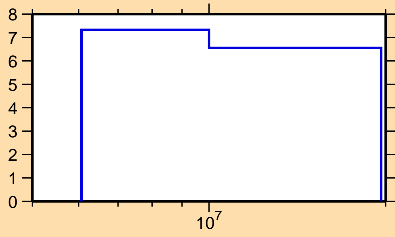
\Delta\sigma/\sigma vs. E for ^{196}\text{Au}(n,\text{nonel.})
