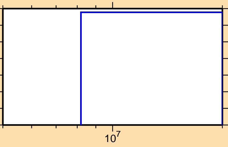
\sigma vs. E for ^{196}\text{Au}(n,3n)
