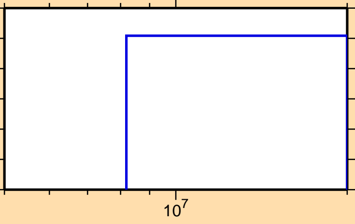
\sigma vs. E for ^{196}\text{Au}(n,nd)
