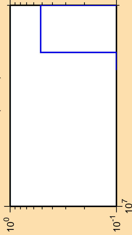
\Delta\sigma/\sigma vs. E for ^{196}\text{Au}(n,3n\alpha)
