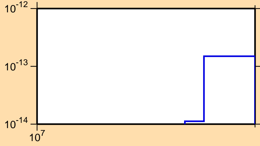
\sigma vs. E for ^{196}\text{Au}(\text{mt117})
