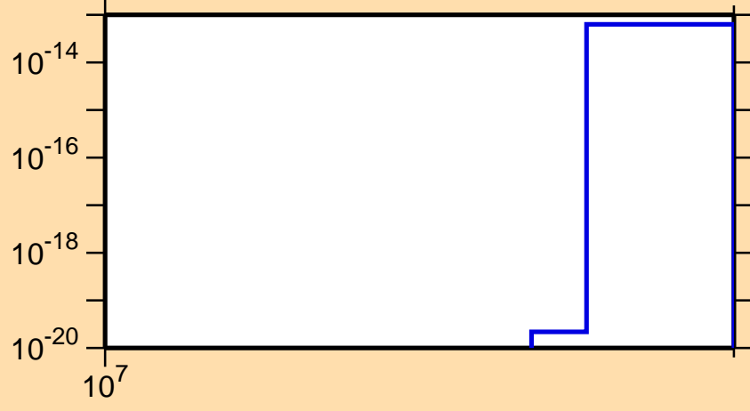
\sigma vs. E for ^{196}\text{Au}(n,3n\alpha)
