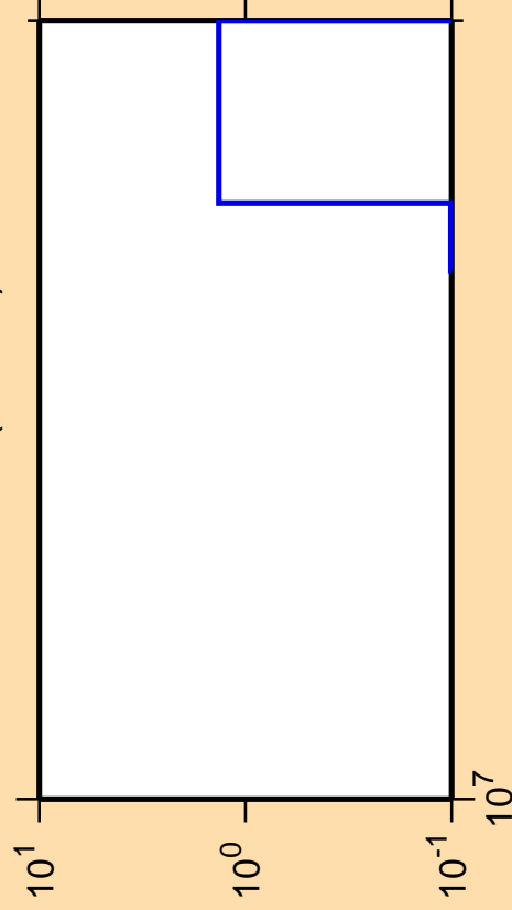
\Delta\sigma/\sigma vs. E for ^{196}\text{Au}(\text{mt117})
