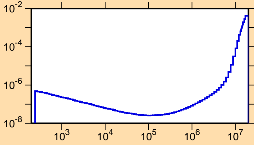
\sigma vs. E for ^{196}\text{Au}(n,\alpha)
