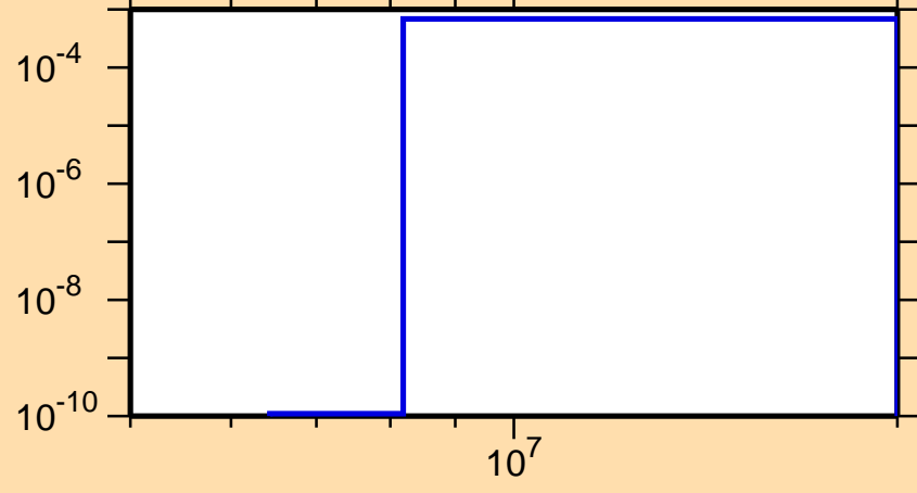
\sigma vs. E for ^{196}\text{Au}(n,d)
