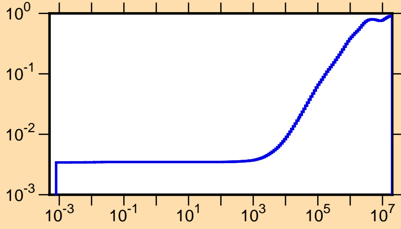
\mu vs. E for ^{197}\text{Au}(\text{mt251})
