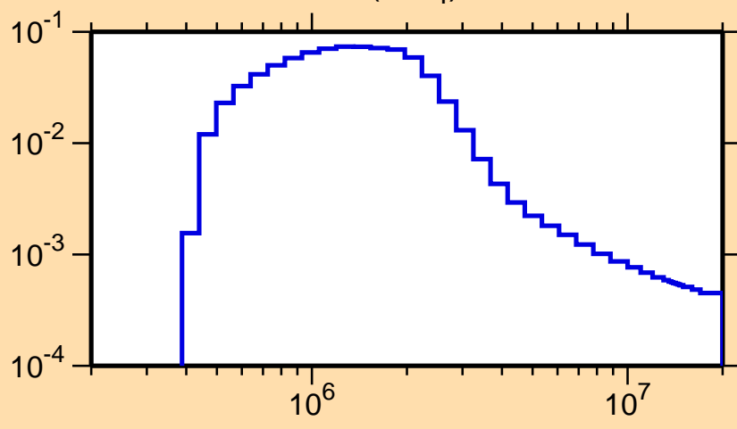
\sigma vs. E for ^{197}\text{Au}(n,n_4)
