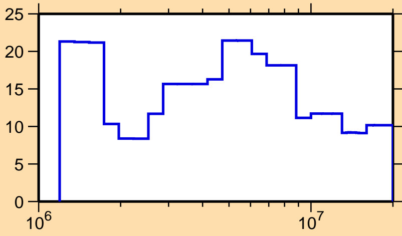
\Delta\sigma/\sigma vs. E for ^{197}\text{Au}(n, el.)
