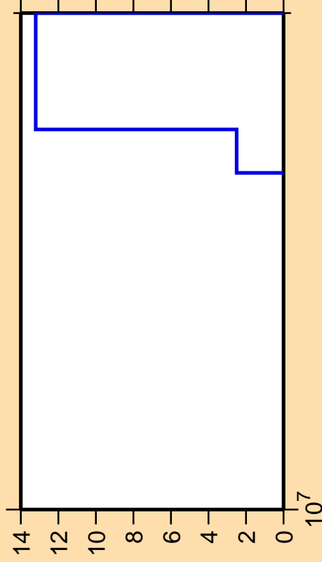
\Delta\sigma/\sigma vs. E for ^{197}\text{Au}(n,p\alpha)
