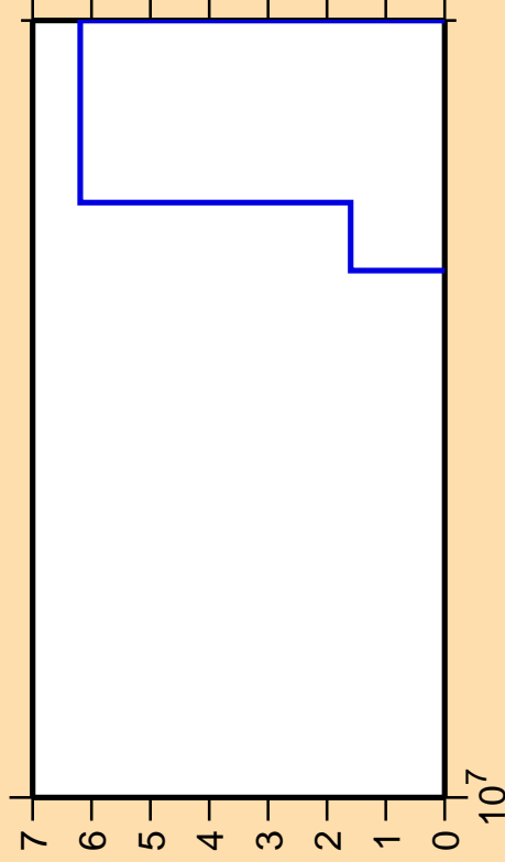
\Delta\sigma/\sigma vs. E for ^{198}\text{Au}(n,p\alpha)
