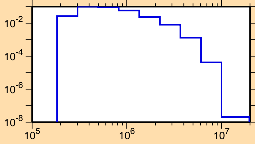
\sigma vs. E for ^{198}\text{Au}(n,n_4)
