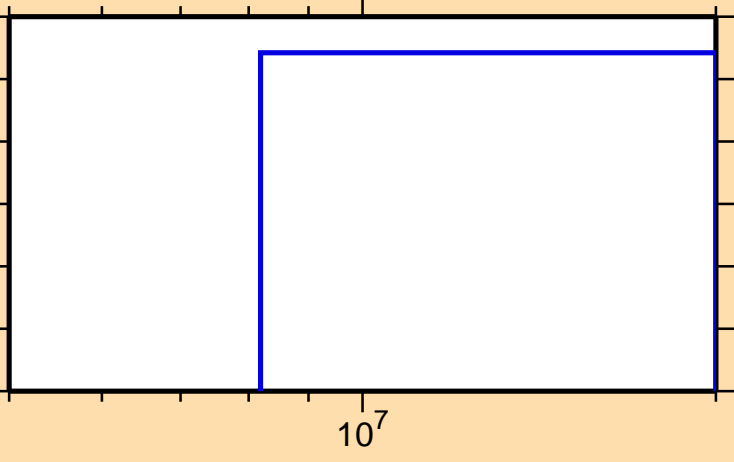
\sigma vs. E for ^{198}\text{Au}(n,2n\alpha)
