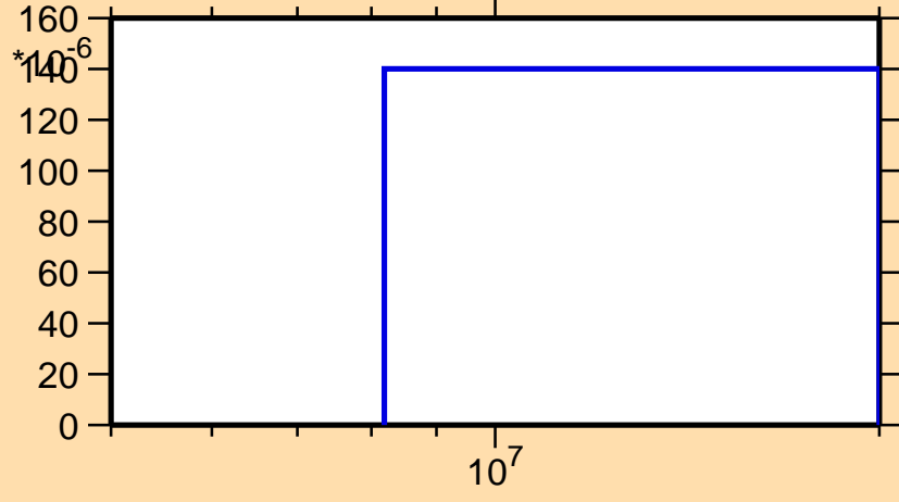
\sigma vs. E for ^{198}\text{Au}(n,np)
