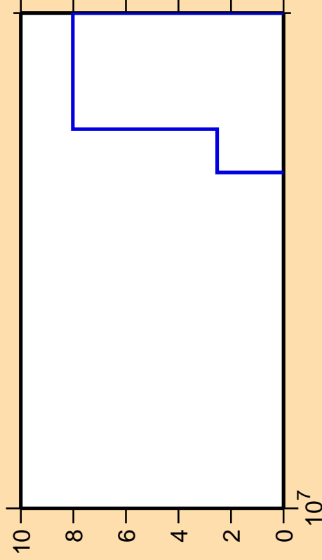
\Delta\sigma/\sigma vs. E for ^{198}\text{Au}(n,p\alpha)
