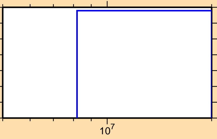
\sigma vs. E for ^{198}\text{Au}(n,2n\alpha)
