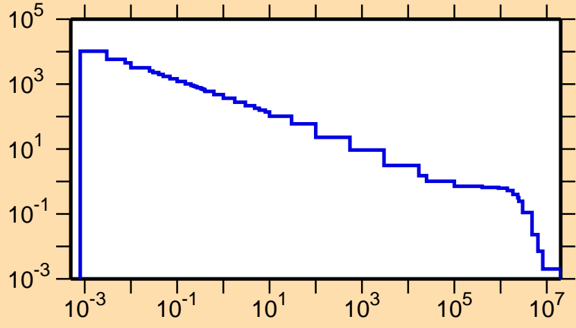
\sigma vs. E for ^{198}\text{Au}(n,\gamma)
