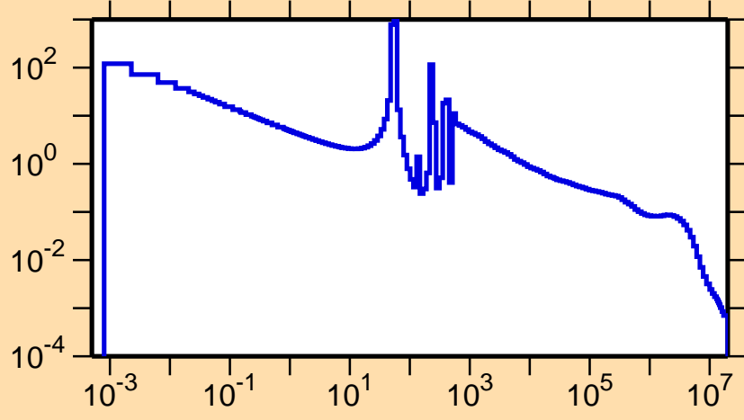
\sigma vs. E for ^{199}\text{Au}(n,\gamma)
