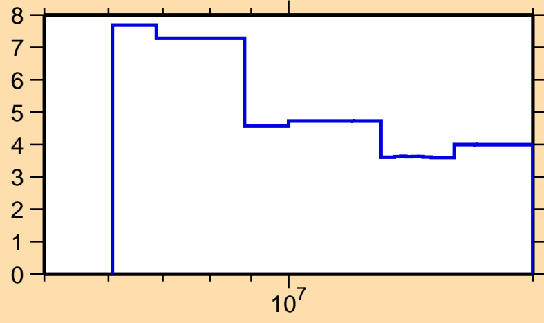
\Delta\sigma/\sigma vs. E for ^{200}\text{Au}(n,\text{tot.})
