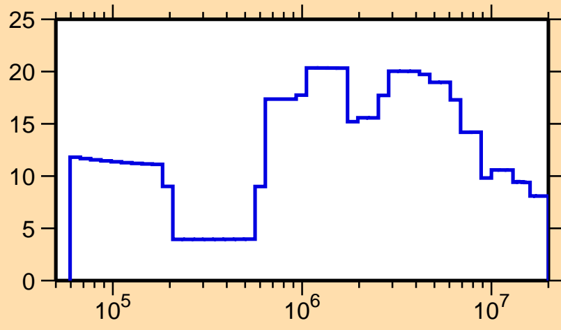
\Delta\sigma/\sigma vs. E for ^{200}\text{Au}(n,\text{el.})
