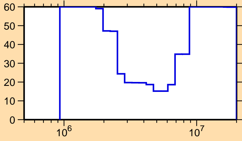
\Delta\sigma/\sigma vs. E for ^{200}\text{Au}(n,n\text{cont.})
