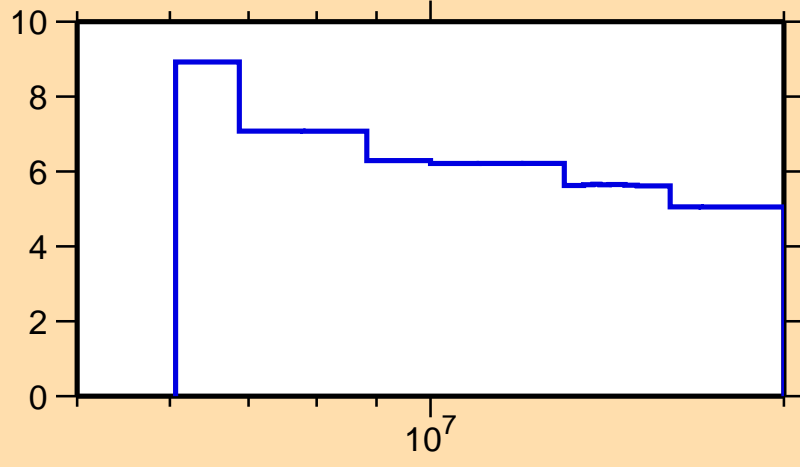
\Delta\sigma/\sigma vs. E for ^{200}\text{Au}(n,\text{nonel.})
