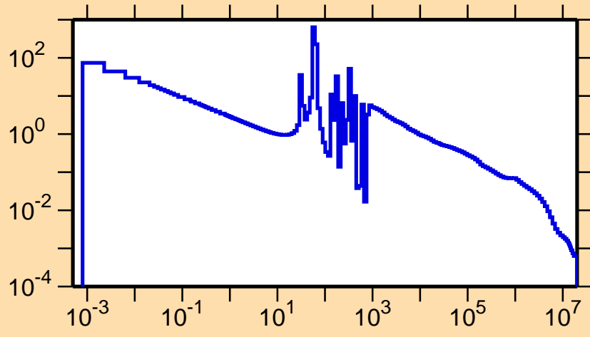
\sigma vs. E for ^{200}\text{Au}(n,\gamma)
