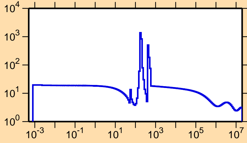
\sigma vs. E for ^{200}\text{Au}(n,\text{el.})
