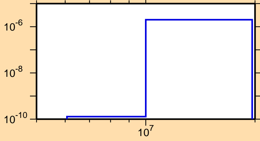
\sigma vs. E for ^{200}\text{Au}(n,n\alpha)
