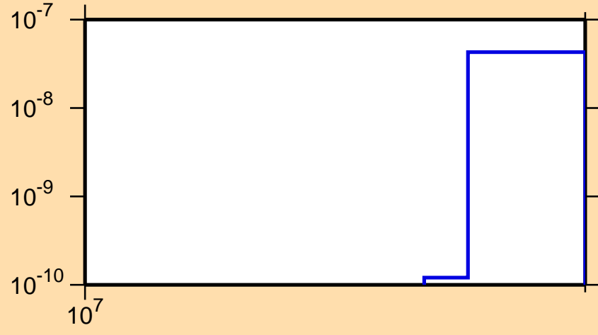
\sigma vs. E for ^{201}\text{Au}(n,nd)
