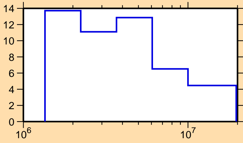
\Delta\sigma/\sigma vs. E for ^{201}\text{Au}(n,\text{tot.})
