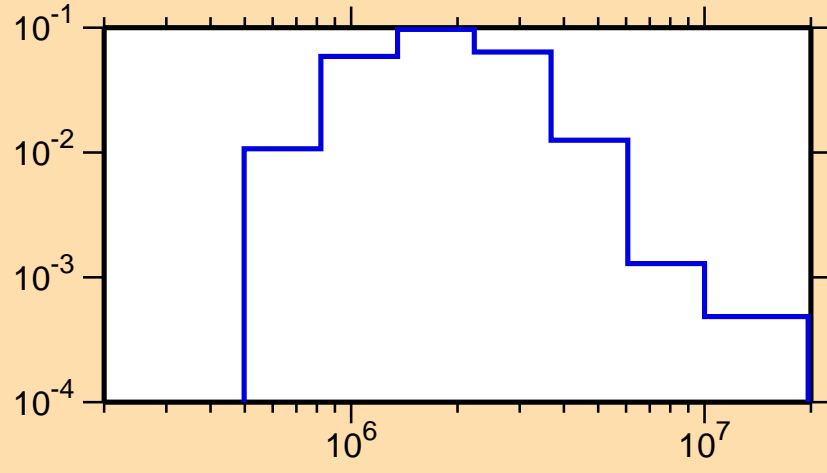
\sigma vs. E for ^{201}\text{Au}(n,n_4)
