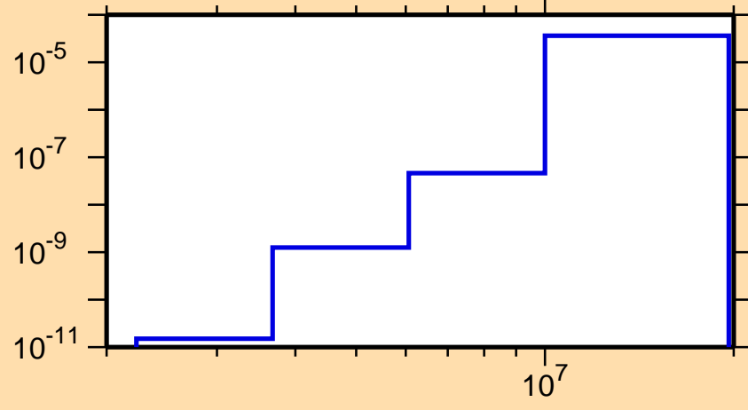
\sigma vs. E for ^{201}\text{Au}(n,\alpha)
