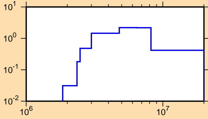
\sigma vs. E for ^{201}\text{Au}(n,n\text{cont.})
