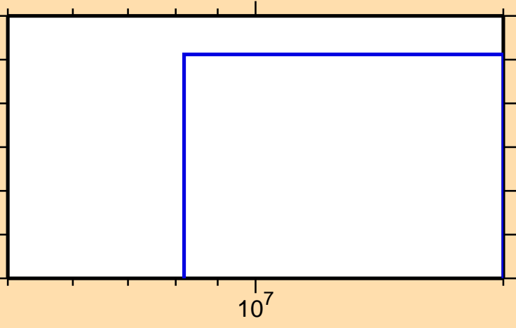
\sigma vs. E for ^{201}\text{Au}(n,nt)
