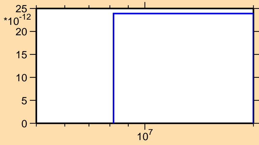
\sigma vs. E for ^{201}\text{Au}(n,2n\alpha)
