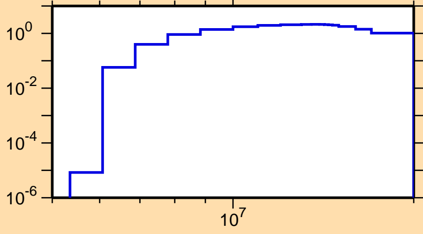
\sigma vs. E for ^{202}\text{Au}(n,2n)
