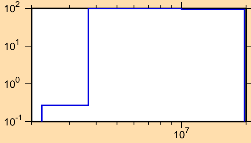
\Delta\sigma/\sigma vs. E for ^{202}\text{Au}(n,p)
