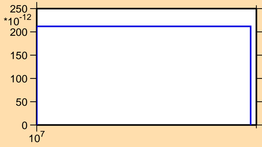
\sigma vs. E for ^{202}\text{Au}(n,nt)
