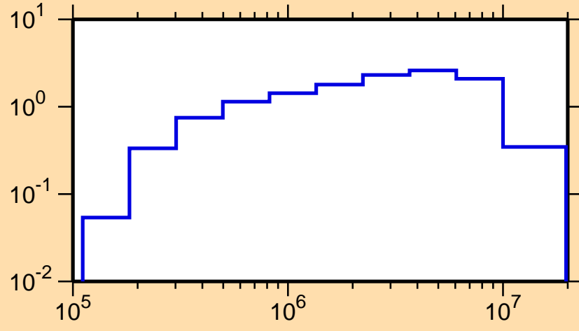
\sigma vs. E for ^{202}\text{Au}(n,\text{inel.})
