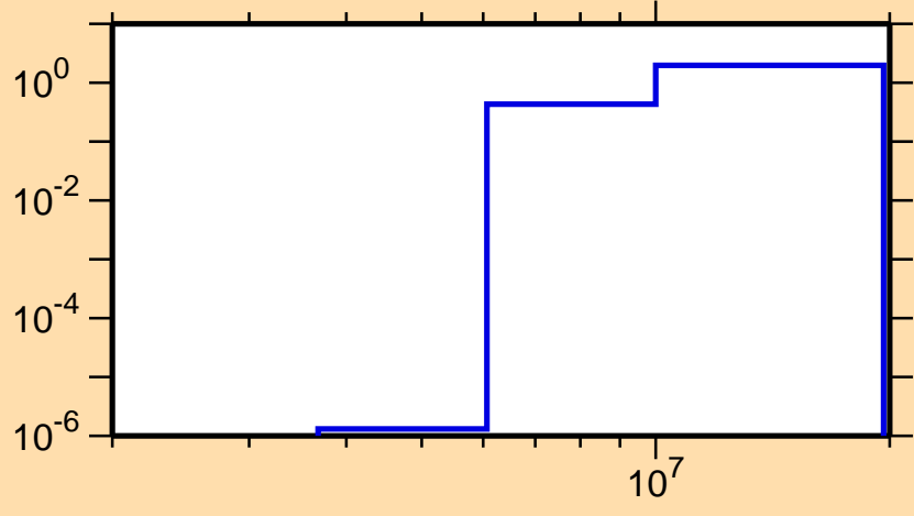
\sigma vs. E for ^{202}\text{Au}(n,2n)
