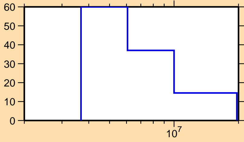
\Delta\sigma/\sigma vs. E for ^{202}\text{Au}(n,2n)
