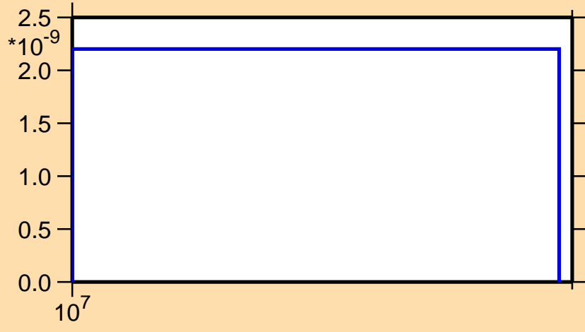
\sigma vs. E for ^{202}\text{Au}(n,\text{nd})
