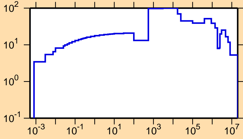
\Delta\sigma/\sigma vs. E for ^{202}\text{Au}(n,\text{tot.})
