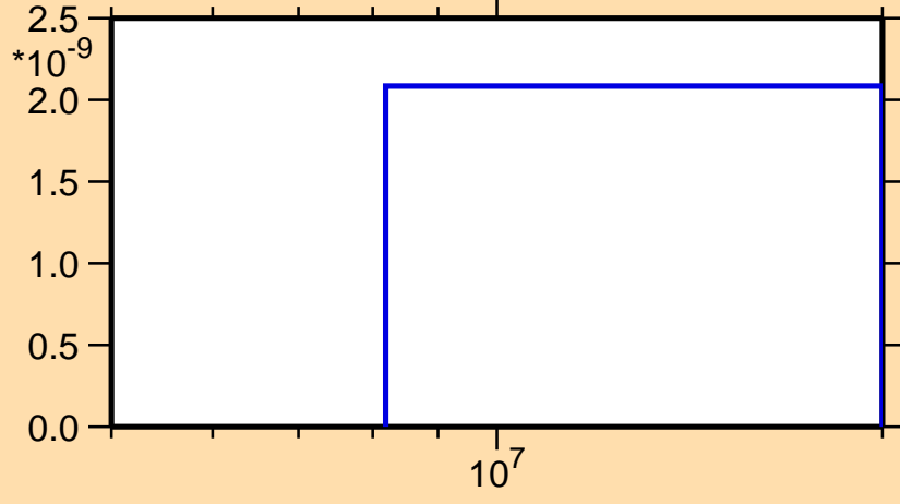
\sigma vs. E for ^{202}\text{Au}(n,nd)
