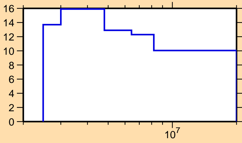
\Delta\sigma/\sigma vs. E for ^{202}\text{Au}(n,\text{nonel.})
