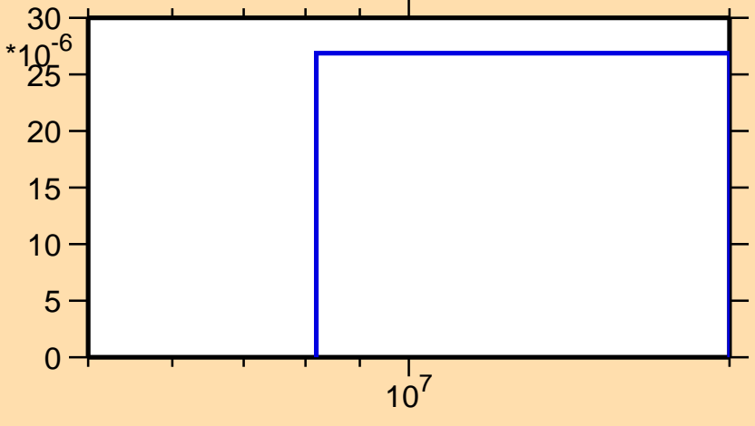
\sigma vs. E for ^{202}\text{Au}(n,d)
