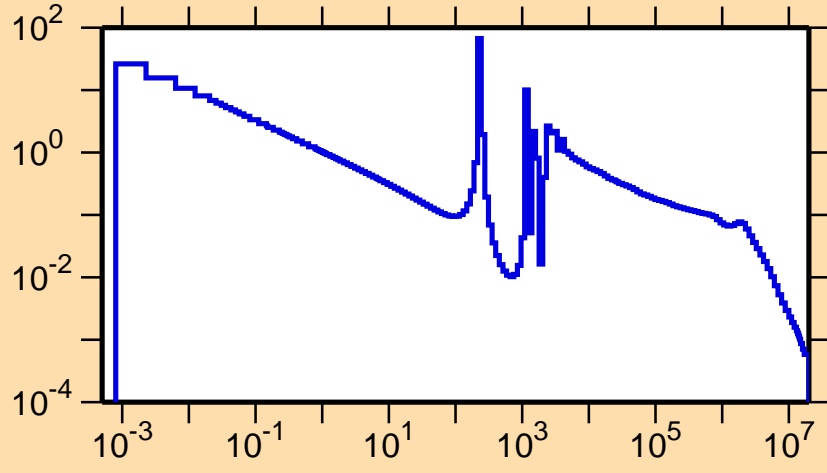
\sigma vs. E for ^{203}\text{Au}(n,\gamma)
