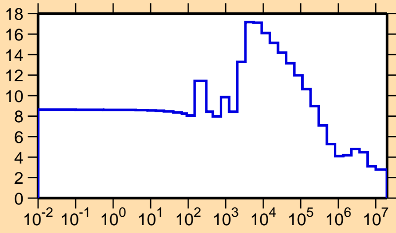
\sigma vs. E for ^{203}\text{Au}(n,\text{el.})
