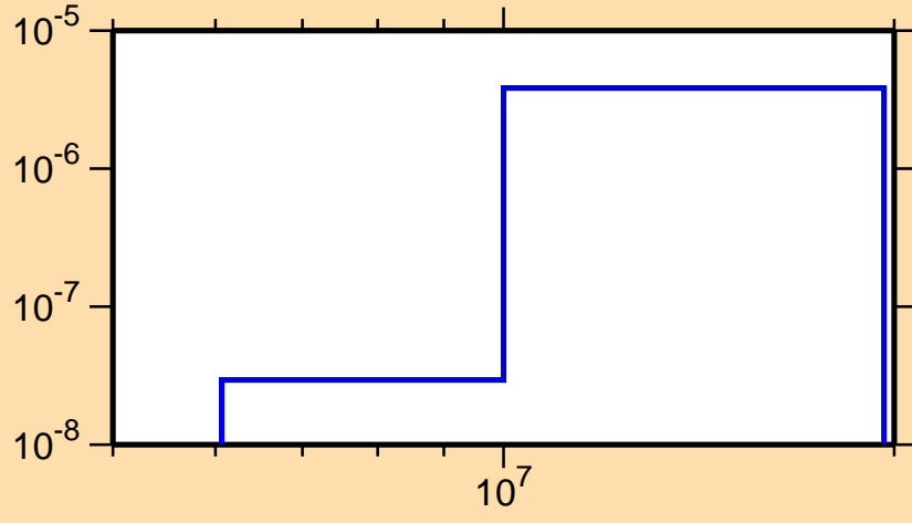
\sigma vs. E for ^{203}\text{Au}(n,n\alpha)
