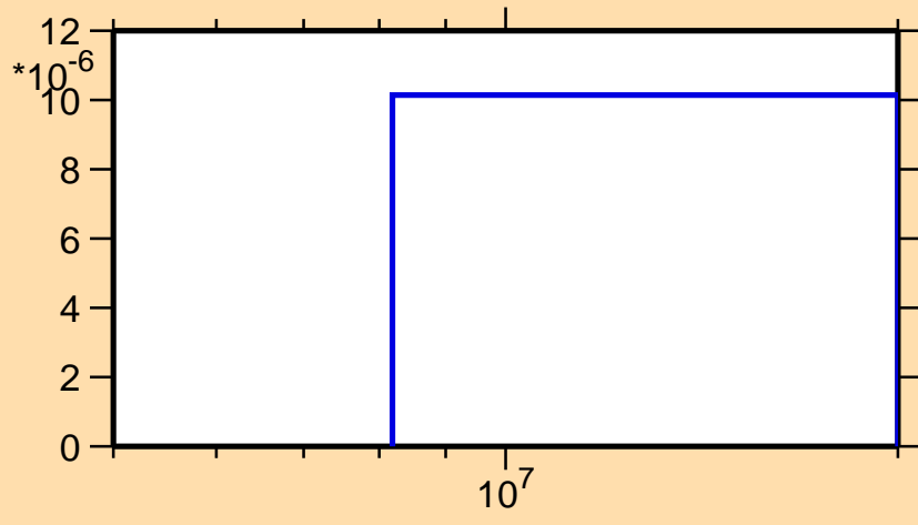
\sigma vs. E for ^{203}\text{Au}(n,np)
