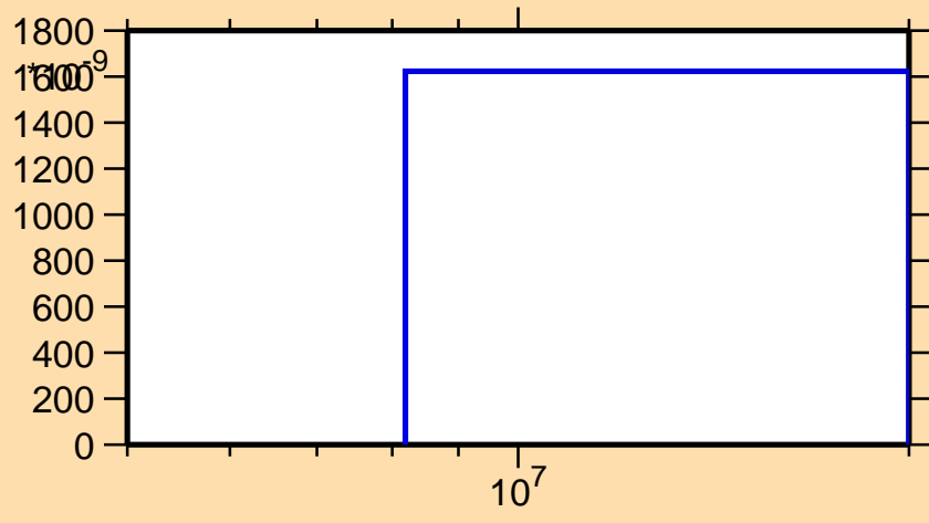
\sigma vs. E for ^{203}\text{Au}(n,t)
