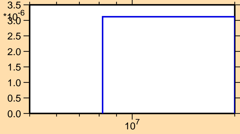
\sigma vs. E for ^{203}\text{Au}(n,n\alpha)
