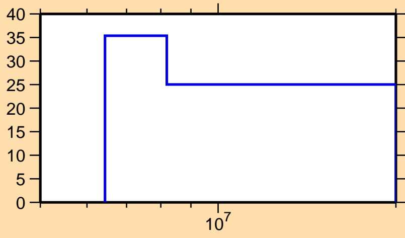
\Delta\sigma/\sigma vs. E for ^{203}\text{Au}(n,\text{el.})
