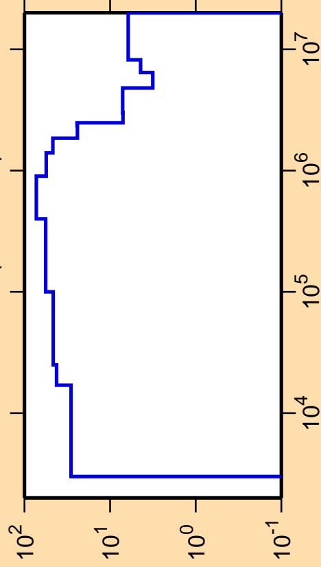
\Delta\sigma/\sigma vs. E for ^{203}\text{Au}(n,\text{nonel.})
