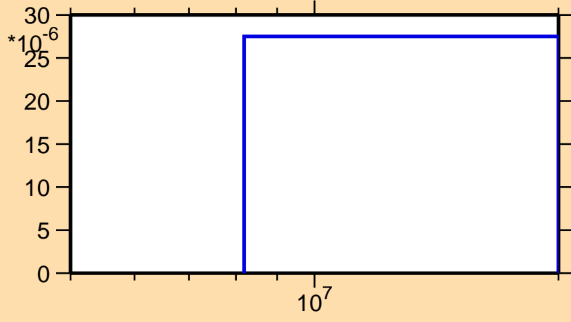
\sigma vs. E for ^{203}\text{Au}(n,d)
