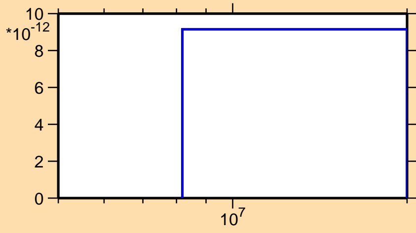
\sigma vs. E for ^{203}\text{Au}(n,2n\alpha)
