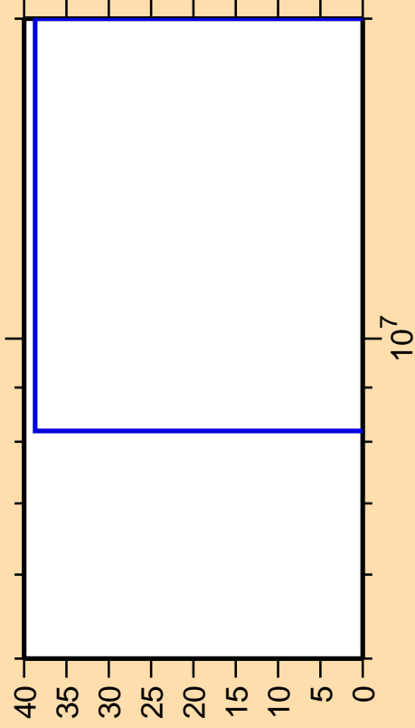
\Delta\sigma/\sigma vs. E for ^{203}\text{Au}(n,2n\alpha)
