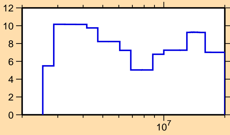
\Delta\sigma/\sigma vs. E for ^{204}\text{Au}(n,\text{nonel.})
