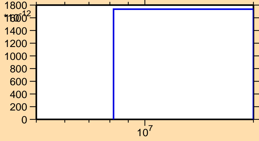
\sigma vs. E for ^{204}\text{Au}(n,nd)
