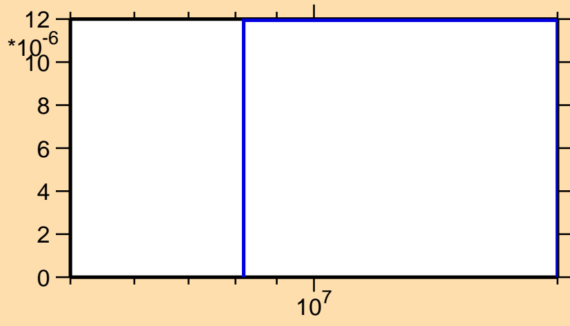
\sigma vs. E for ^{204}\text{Au}(n,np)
