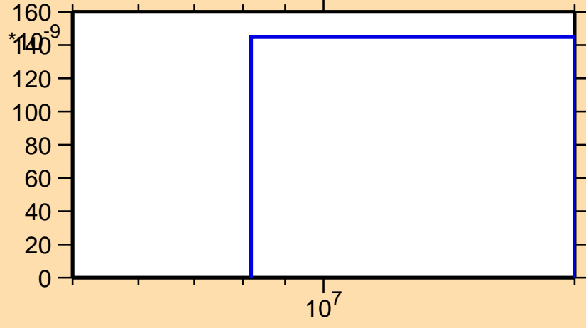
\sigma vs. E for ^{204}\text{Au}(n,n\alpha)
