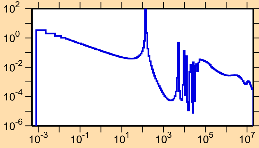
\sigma vs. E for ^{205}\text{Au}(n,\gamma)
